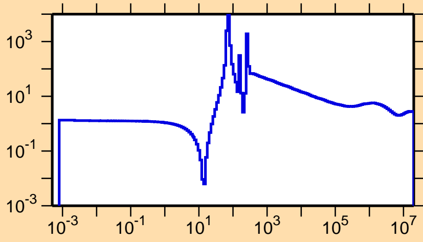
\sigma vs. E for ^{140}\text{Nd}(n,\text{el.})
