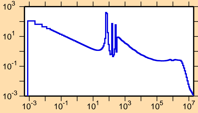
\sigma vs. E for ^{140}\text{Nd}(n,\gamma)
