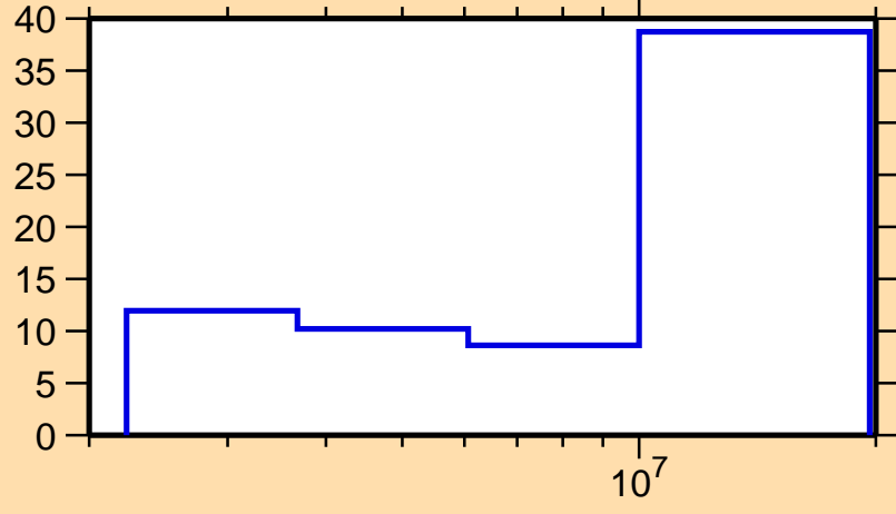
\Delta\sigma/\sigma vs. E for ^{140}\text{Nd}(n,n\text{cont.})
