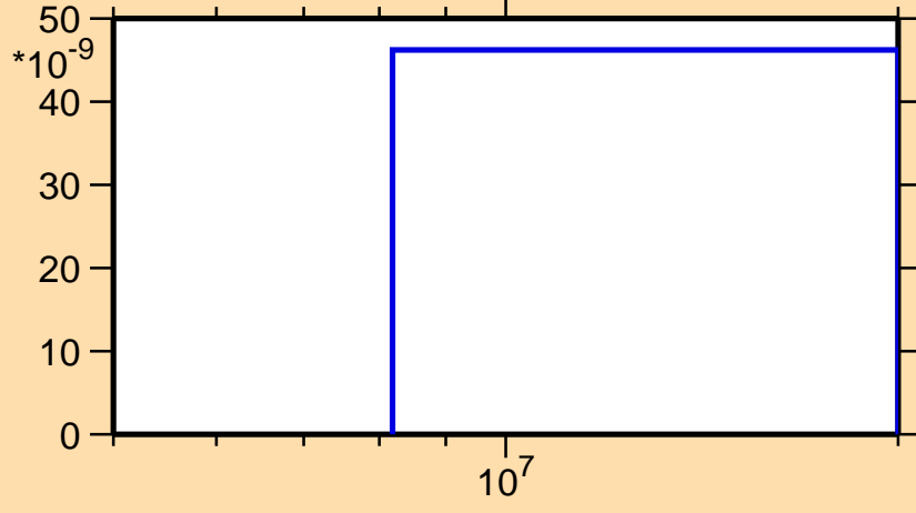
\sigma vs. E for ^{140}\text{Nd}(n,p\alpha)
