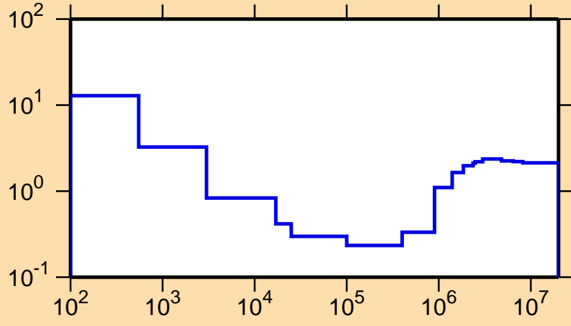
\sigma vs. E for ^{140}\text{Nd}(n,\text{nonel.})
