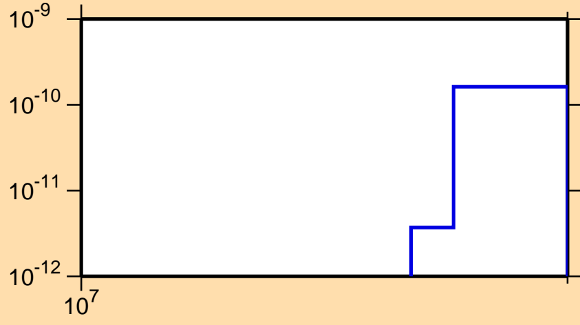
\sigma vs. E for ^{141}\text{Nd}(n,\text{pd})
