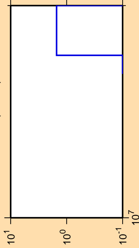
\Delta\sigma/\sigma vs. E for ^{141}\text{Nd} (mt 34)
