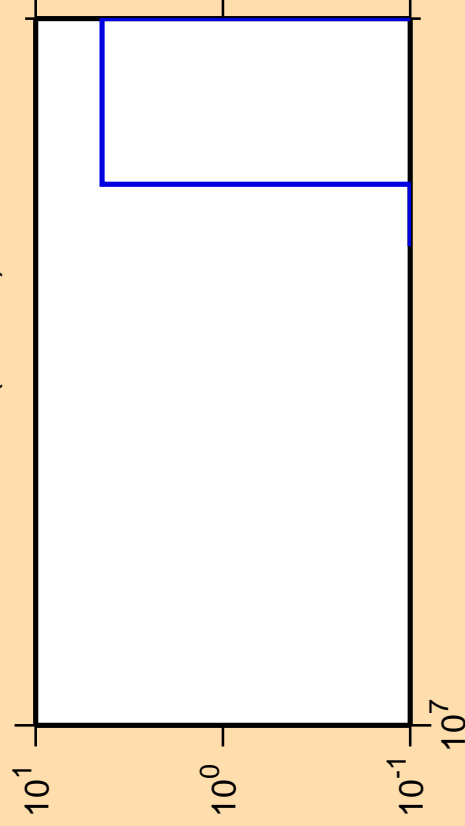
\Delta\sigma/\sigma vs. E for ^{141}\text{Nd} (mt 45)
