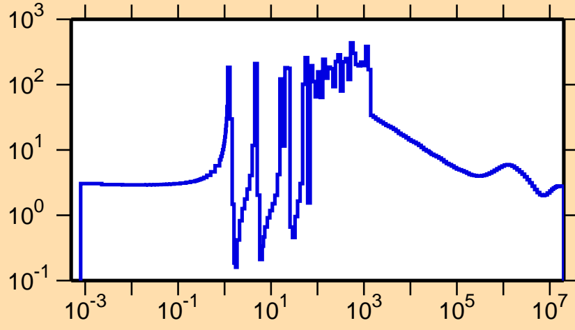
\sigma vs. E for ^{141}\text{Nd}(n,\text{el.})
