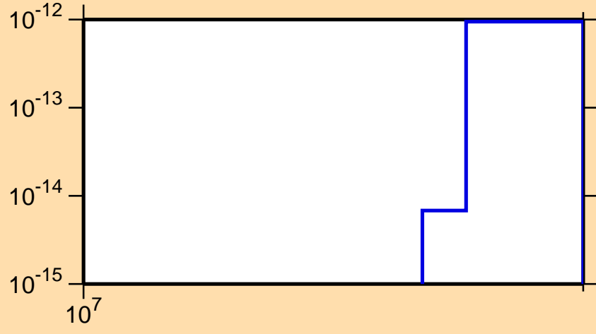
\sigma vs. E for ^{141}\text{Nd}(n,nt)
