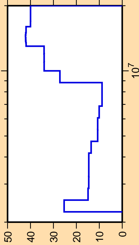
\Delta\sigma/\sigma vs. E for ^{141}\text{Nd}(n,n\text{cont.})
