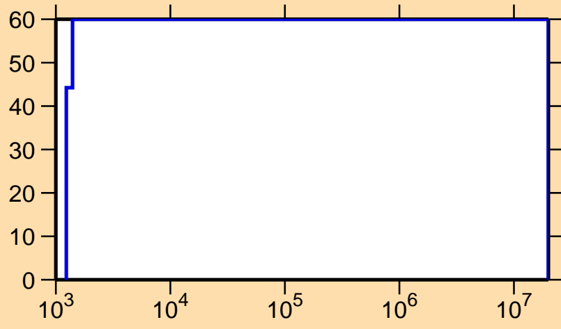
\Delta\sigma/\sigma vs. E for ^{141}\text{Nd}(n,\gamma)
