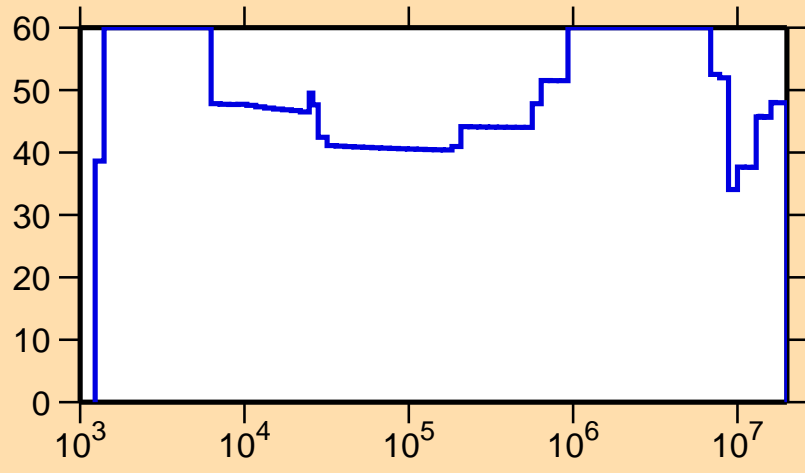
\Delta\sigma/\sigma vs. E for ^{141}\text{Nd}(n,p)
