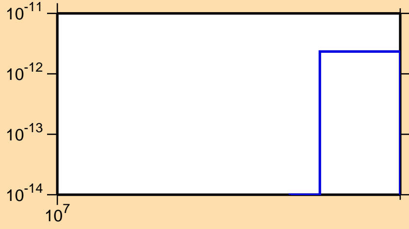
\sigma vs. E for ^{141}\text{Nd} (mt 45)
