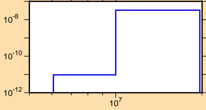
\sigma vs. E for ^{141}\text{Nd}(n,p\alpha)
