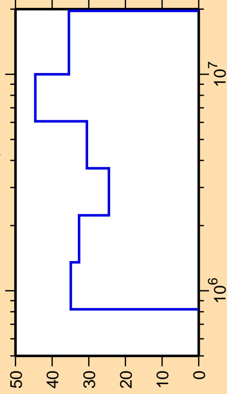
\Delta\sigma/\sigma vs. E for ^{141}\text{Nd}(n,n_3)
