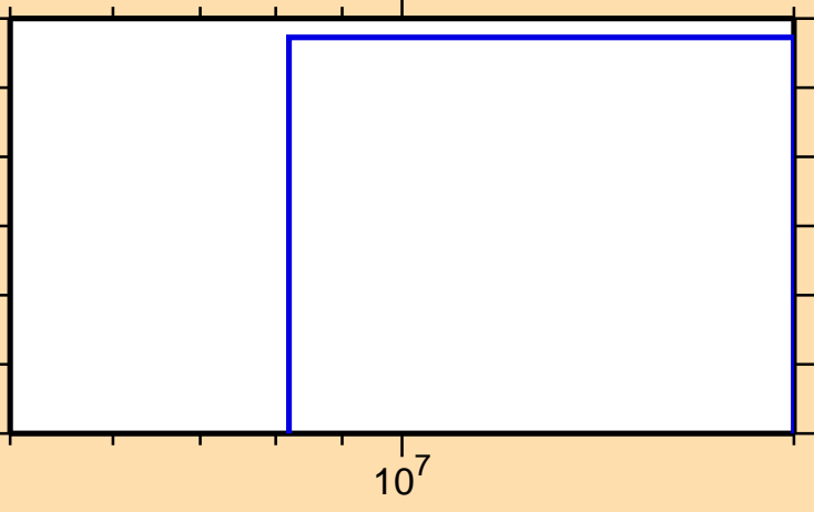
\sigma vs. E for ^{141}\text{Nd}(n,\text{nd})
