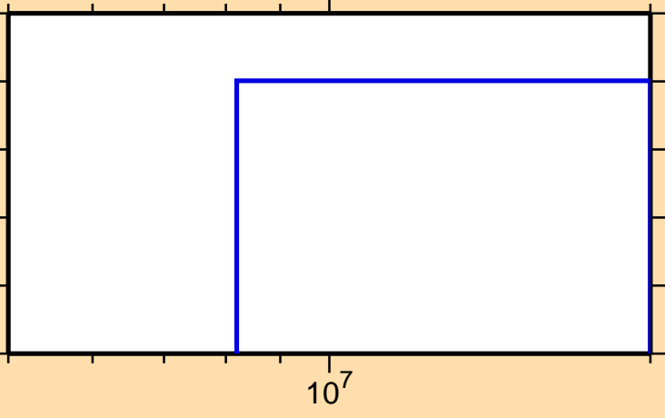
\sigma vs. E for ^{141}\text{Nd}(n,2n\alpha)
