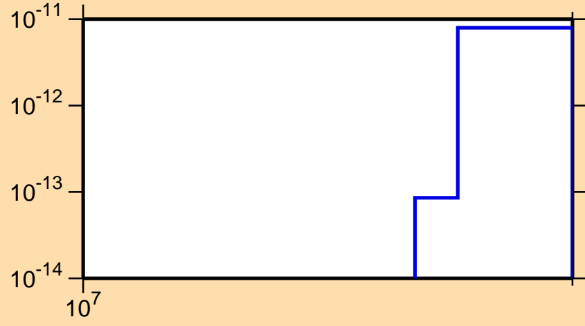
\sigma vs. E for ^{141}\text{Nd} (mt 45)
