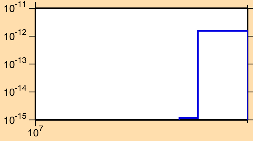
\sigma vs. E for ^{141}\text{Nd} (mt 34)
