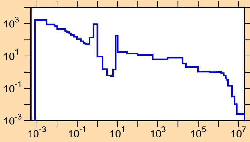
\sigma vs. E for ^{141}\text{Nd}(n,\gamma)
