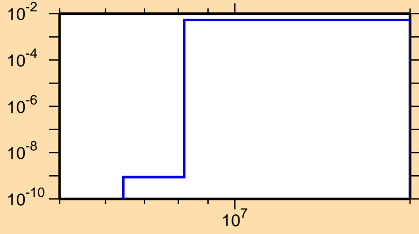
\sigma vs. E for ^{141}\text{Nd}(n,np)
