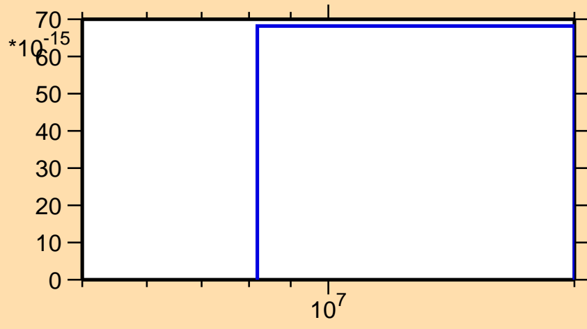
\sigma vs. E for ^{141}\text{Nd}(\text{mt } 45)
