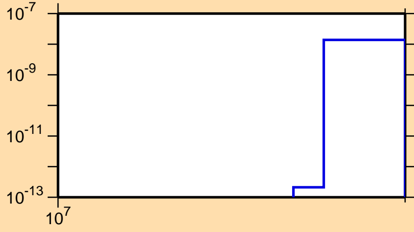
\sigma vs. E for ^{142}\text{Nd}(n,\text{nd})
