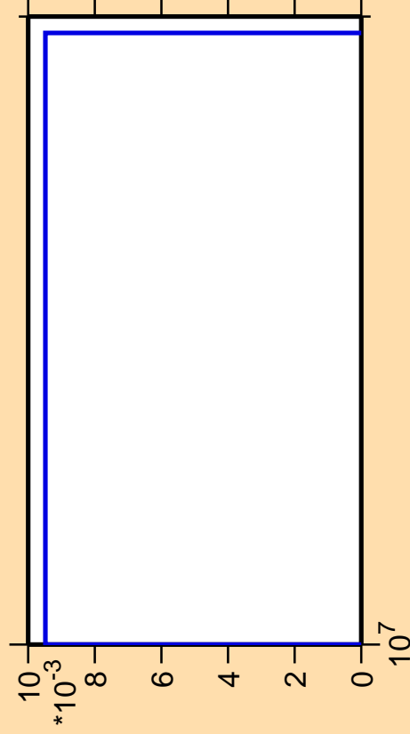
\Delta\sigma/\sigma vs. E for ^{142}\text{Nd} (mt 45)
