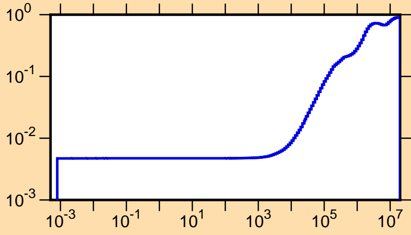
\mu vs. E for ^{143}\text{Nd}(\text{mt251})
