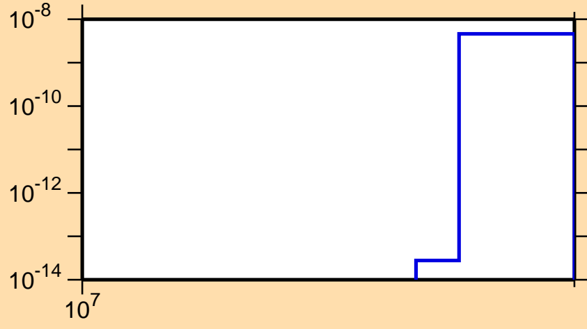
\sigma vs. E for ^{143}\text{Nd}(n,nt)
