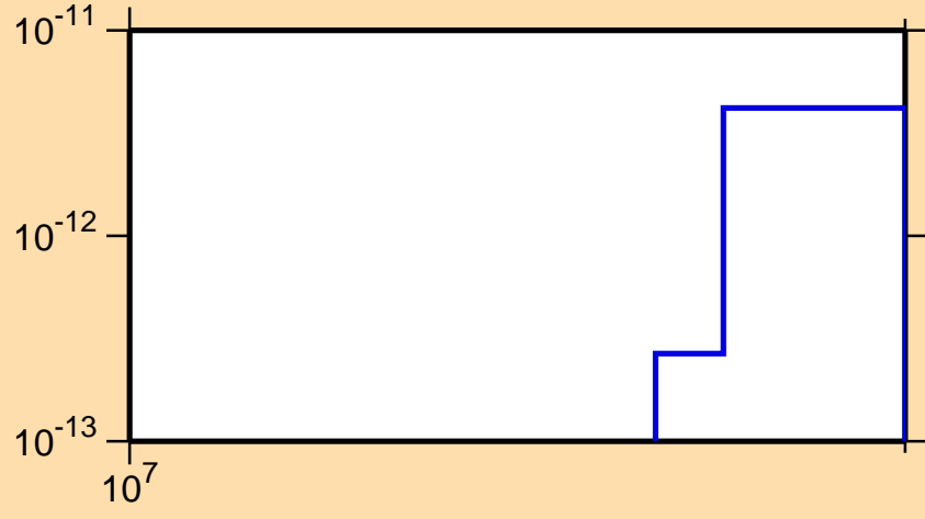
\sigma vs. E for ^{143}\text{Nd}(\text{mt117})
