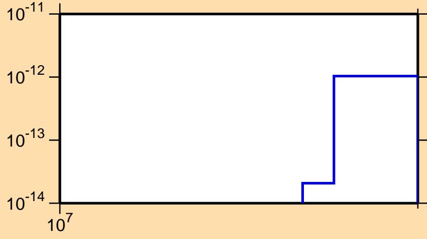
\sigma vs. E for ^{143}\text{Nd} (mt 45)
