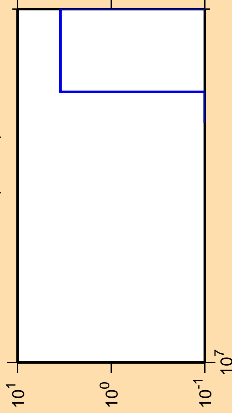
\Delta\sigma/\sigma vs. E for ^{143}\text{Nd} (mt 45)
