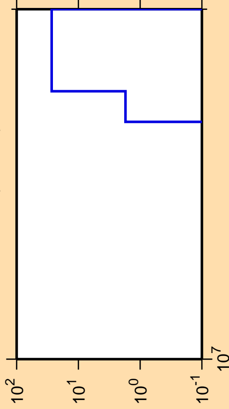
\Delta\sigma/\sigma vs. E for ^{143}\text{Nd}(\text{mt117})
