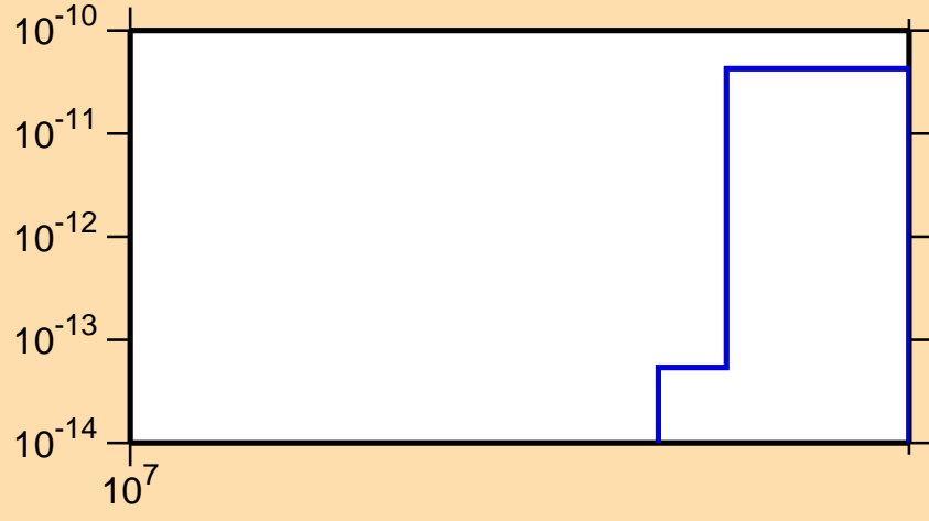
\sigma vs. E for ^{143}\text{Nd}(n,\text{pt})
