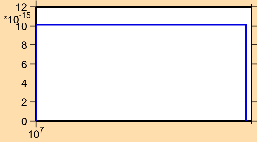
\sigma vs. E for ^{143}\text{Nd} (mt 45)
