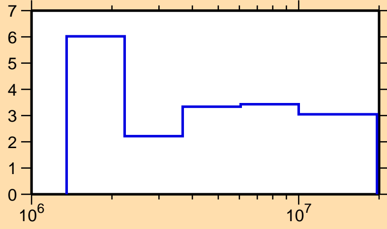
\Delta\sigma/\sigma vs. E for ^{143}\text{Nd}(n,n\text{onel.})
