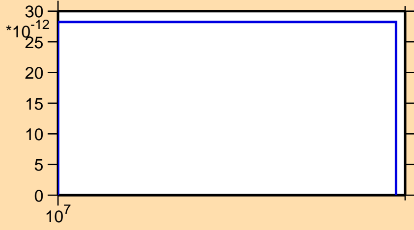
\sigma vs. E for ^{143}\text{Nd}(n,nt)
