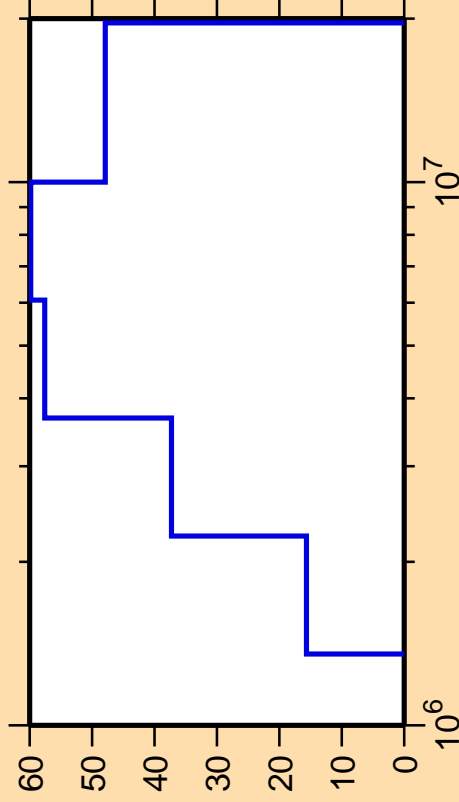
\Delta\sigma/\sigma vs. E for ^{143}\text{Nd}(n,n_4)
