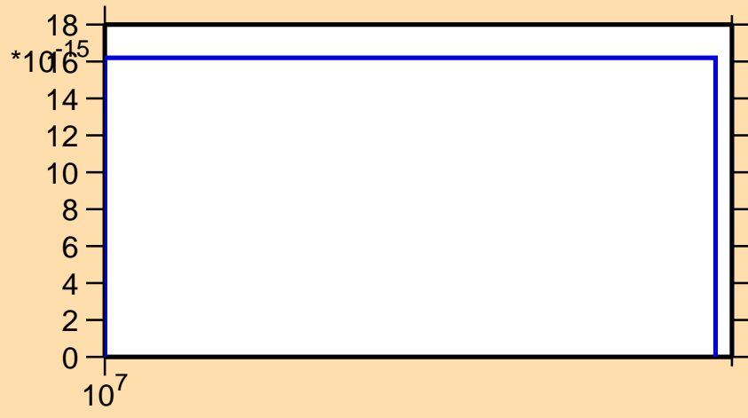
\sigma vs. E for ^{143}\text{Nd} (mt 34)
