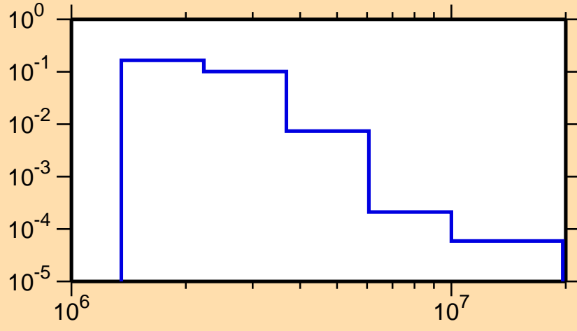
\sigma vs. E for ^{143}\text{Nd}(n,n_4)
