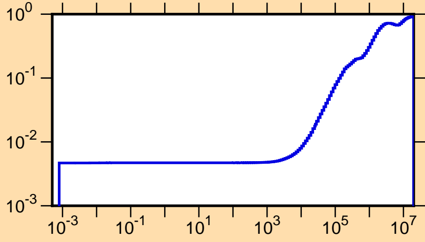
\mu vs. E for ^{144}\text{Nd}(\text{mt251})
