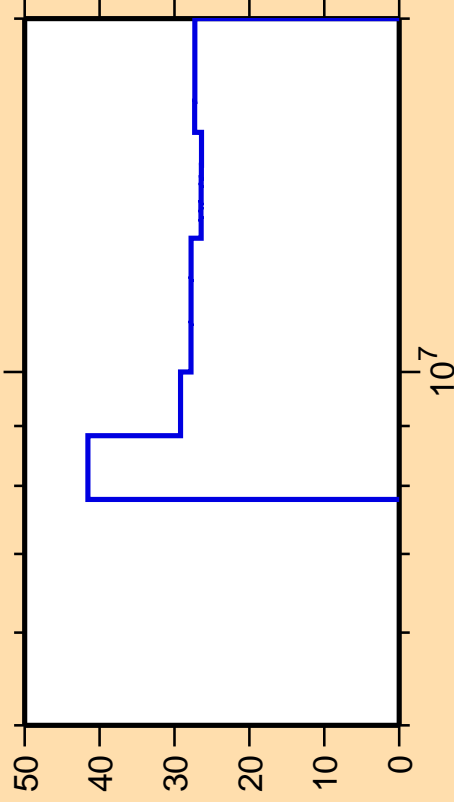
\Delta\sigma/\sigma vs. E for ^{144}\text{Nd}(n,\alpha)
