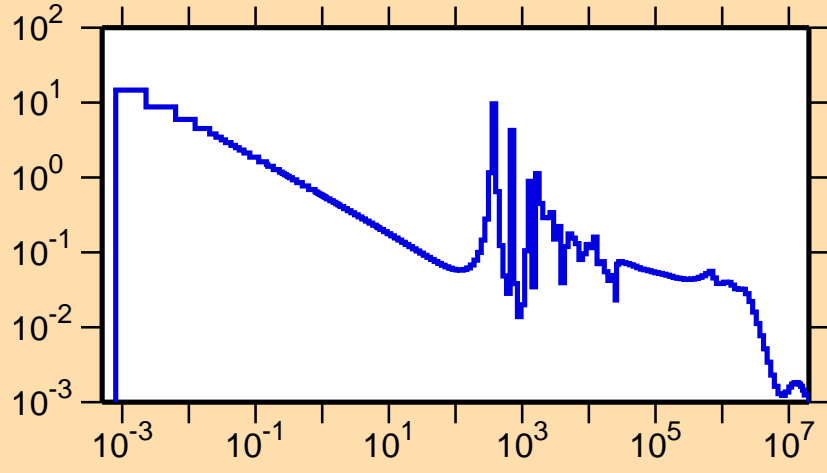
\sigma vs. E for ^{144}\text{Nd}(n,\gamma)
