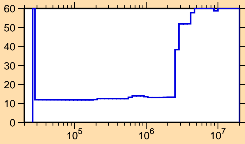
\Delta\sigma/\sigma vs. E for ^{144}\text{Nd}(n,\gamma)
