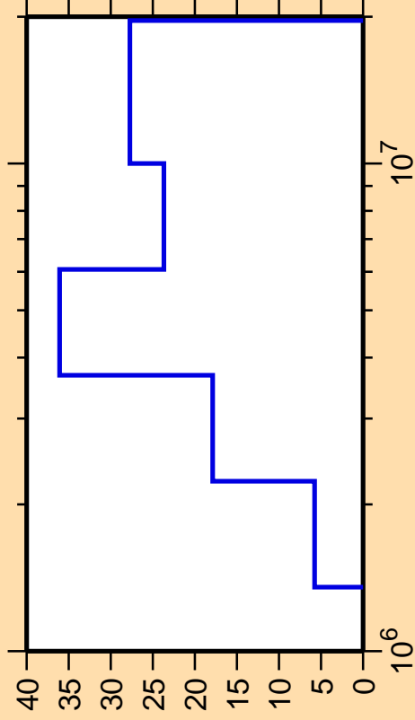
\Delta\sigma/\sigma vs. E for ^{144}\text{Nd}(n,n_4)
