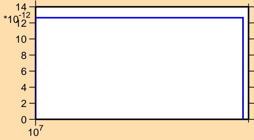
\sigma vs. E for ^{144}\text{Nd} (mt 45)
