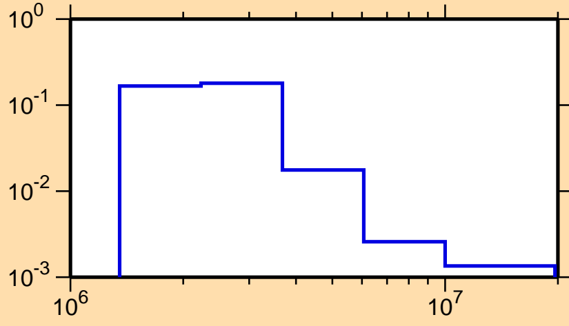
\sigma vs. E for ^{144}\text{Nd}(n,n_4)
