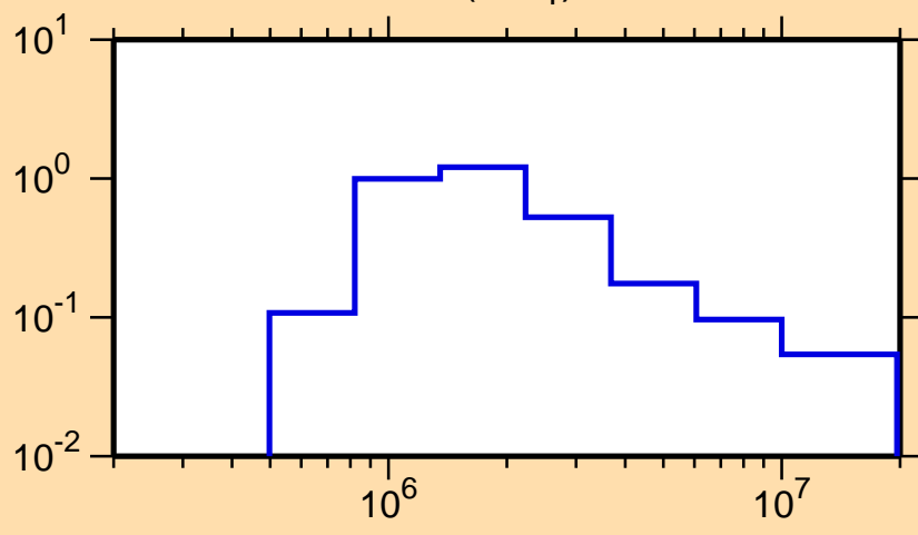
\sigma vs. E for ^{144}\text{Nd}(n,n_1)
