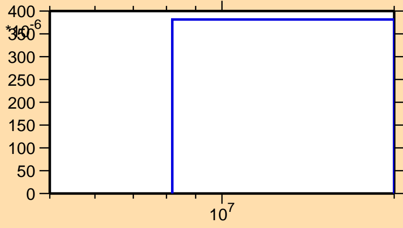
\sigma vs. E for ^{144}\text{Nd}(n,np)
