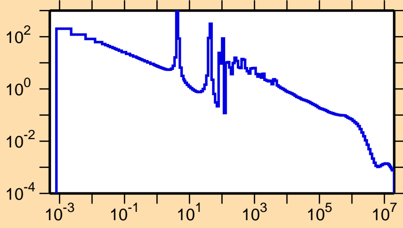
\sigma vs. E for ^{145}\text{Nd}(n,\gamma)
