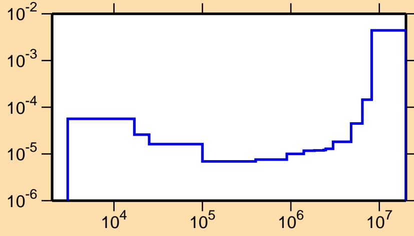
\sigma vs. E for ^{145}\text{Nd}(n,\alpha)
