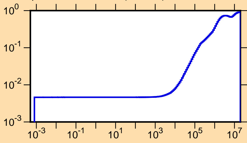
\mu vs. E for ^{146}\text{Nd}(\text{mt251})
