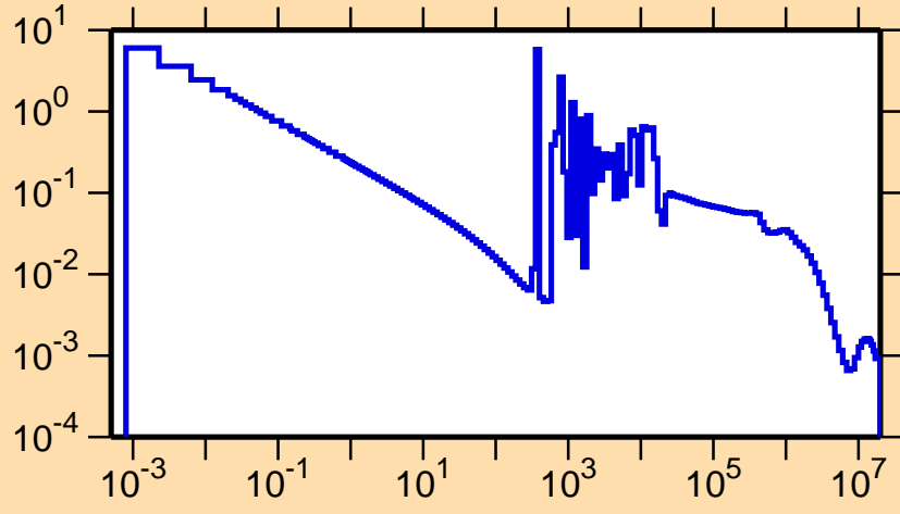
\sigma vs. E for ^{146}\text{Nd}(n,\gamma)
