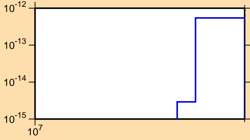
\sigma vs. E for ^{146}\text{Nd} (mt 45)
