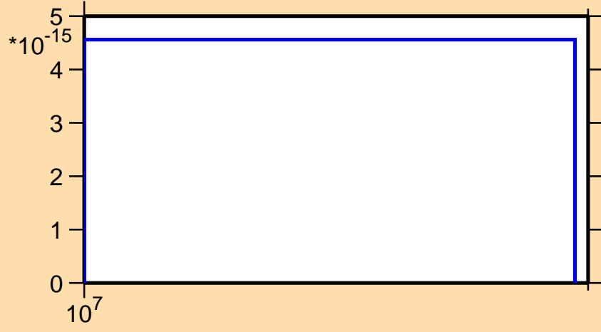
\sigma vs. E for ^{146}\text{Nd} (mt 45)
