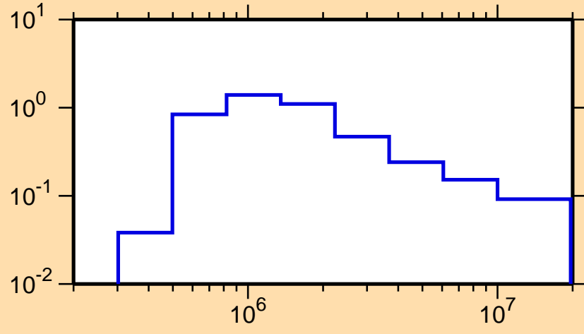
\sigma vs. E for ^{146}\text{Nd}(n,n_1)
