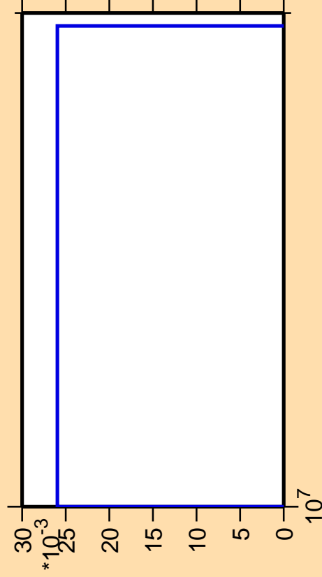
\Delta\sigma/\sigma vs. E for ^{146}\text{Nd} (mt 45)
