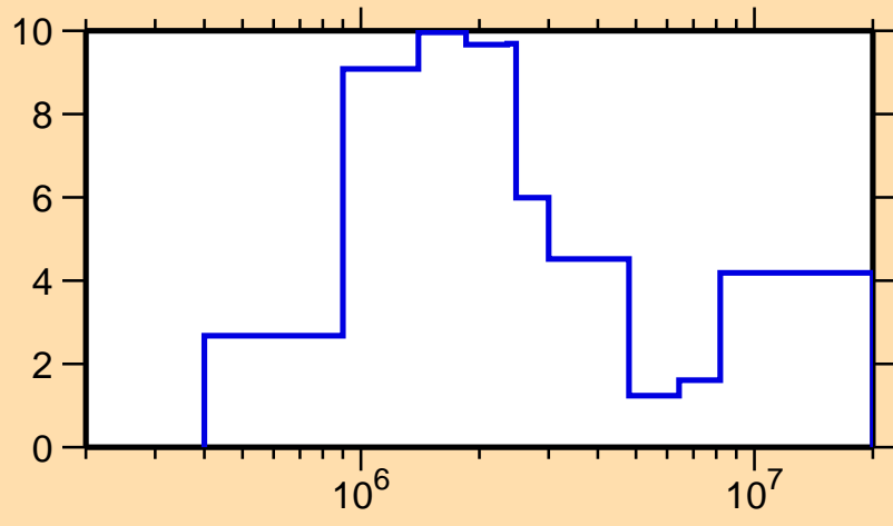
\Delta\sigma/\sigma vs. E for ^{146}\text{Nd}(n,\text{tot.})
