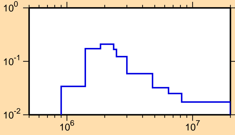
\sigma vs. E for ^{146}\text{Nd}(n,n_3)
