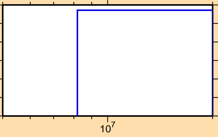
\sigma vs. E for ^{146}\text{Nd}(n,t)
