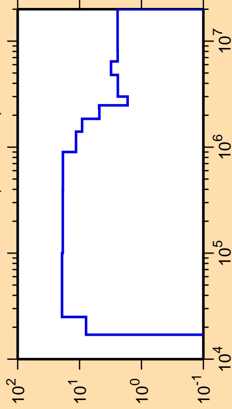
\Delta\sigma/\sigma vs. E for ^{146}\text{Nd}(n,\text{nonel.})
