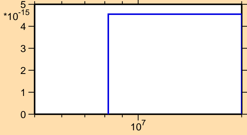
\sigma vs. E for ^{146}\text{Nd}(\text{mt } 45)
