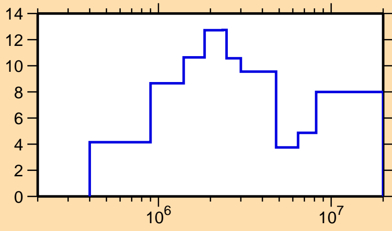
\Delta\sigma/\sigma vs. E for ^{146}\text{Nd}(n,\text{el.})
