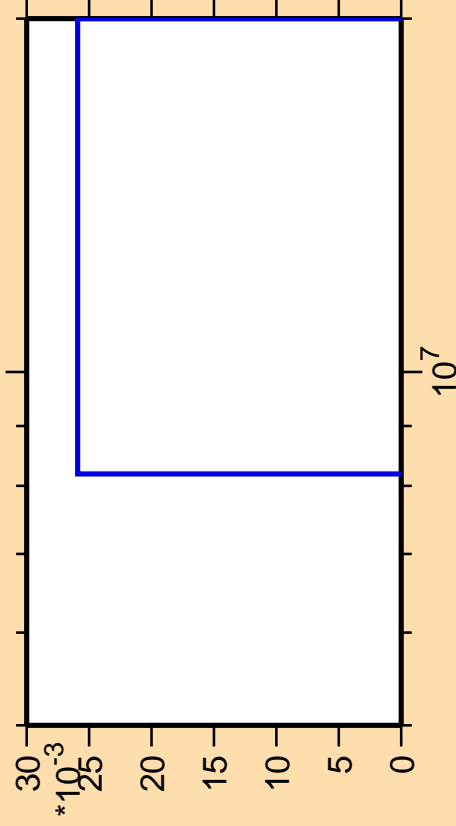
\Delta\sigma/\sigma vs. E for ^{146}\text{Nd}(\text{mt } 45)
