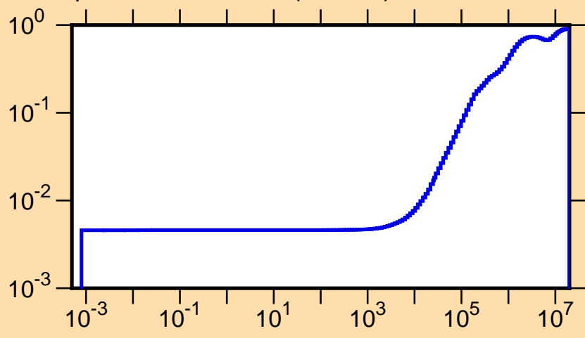
\mu vs. E for ^{147}\text{Nd}(\text{mt251})
