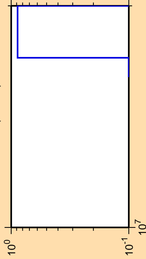
\Delta\sigma/\sigma vs. E for ^{147}\text{Nd} (mt 45)
