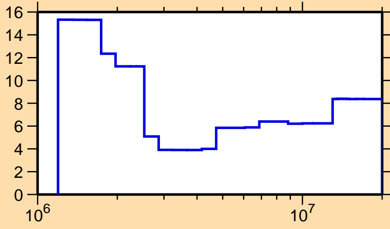
\Delta\sigma/\sigma vs. E for ^{147}\text{Nd}(n,n\text{onel.})
