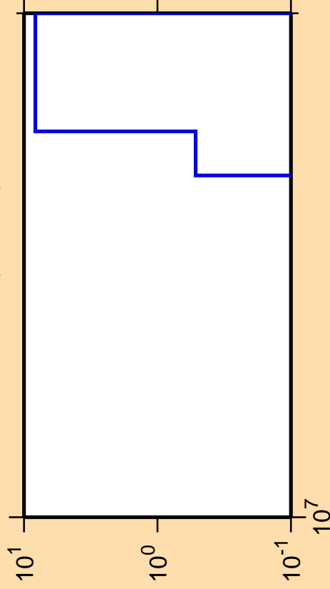
\Delta\sigma/\sigma vs. E for ^{147}\text{Nd}(\text{mt117})
