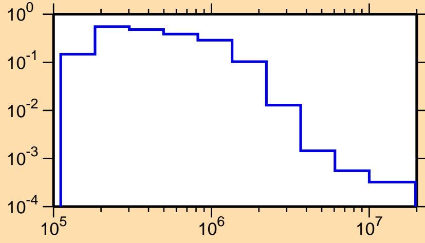
\sigma vs. E for ^{147}\text{Nd}(n,n_2)
