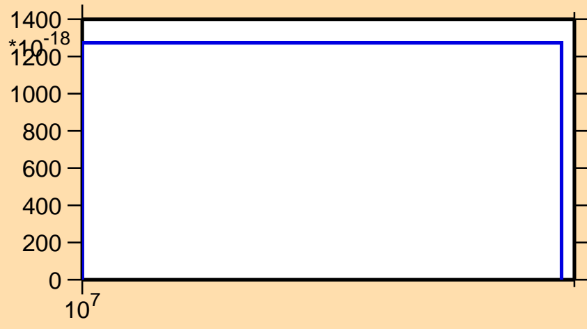
\sigma vs. E for ^{147}\text{Nd} (mt 45)
