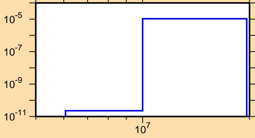
\sigma vs. E for ^{147}\text{Nd}(n,2n\alpha)
