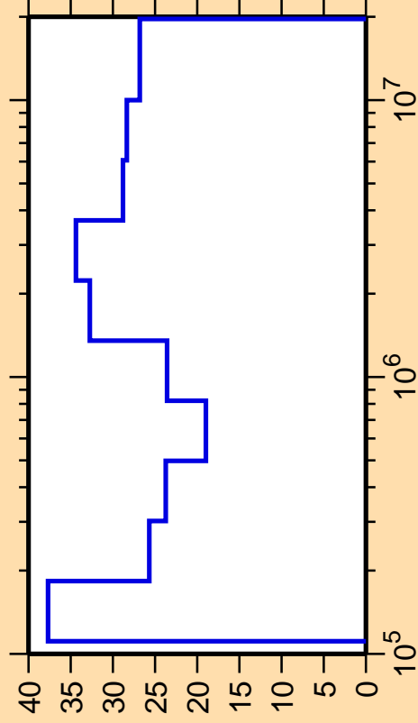
\Delta\sigma/\sigma vs. E for ^{147}\text{Nd}(n,n_2)
