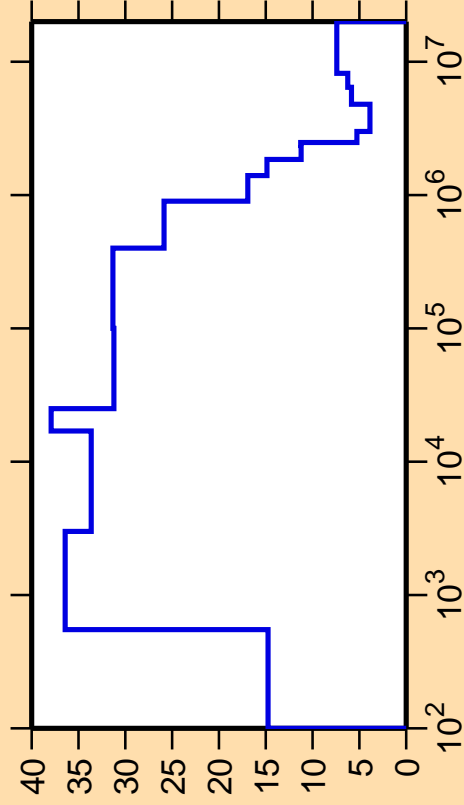
\Delta\sigma/\sigma vs. E for ^{147}\text{Nd}(n,\text{nonel.})
