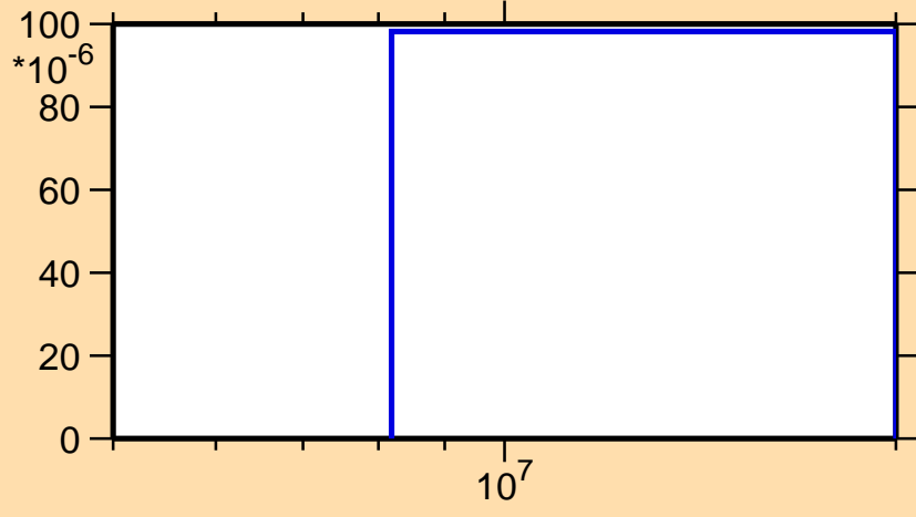
\sigma vs. E for ^{147}\text{Nd}(n,np)
