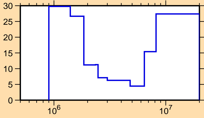
\Delta\sigma/\sigma vs. E for ^{147}\text{Nd}(n,n\text{cont.})
