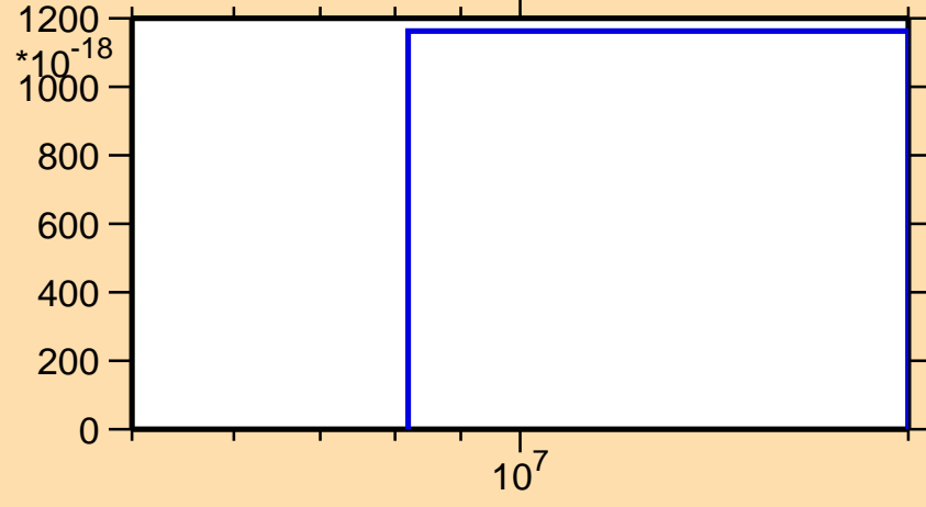
\sigma vs. E for ^{147}\text{Nd}(\text{mt } 45)
