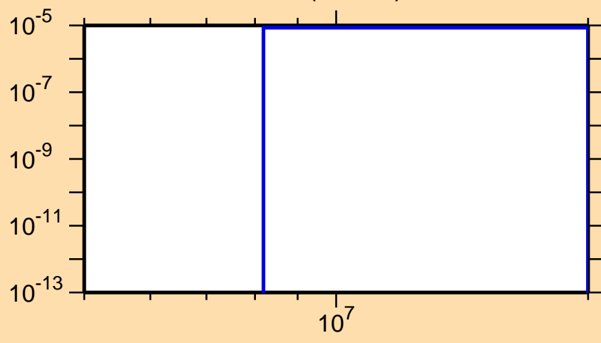
\sigma vs. E for ^{147}\text{Nd}(n,2n\alpha)
