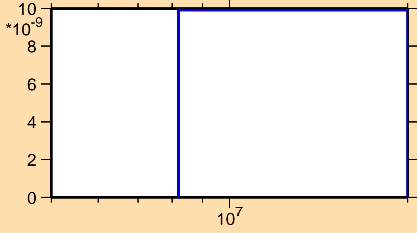
\sigma vs. E for ^{147}\text{Nd}(n,nt)
