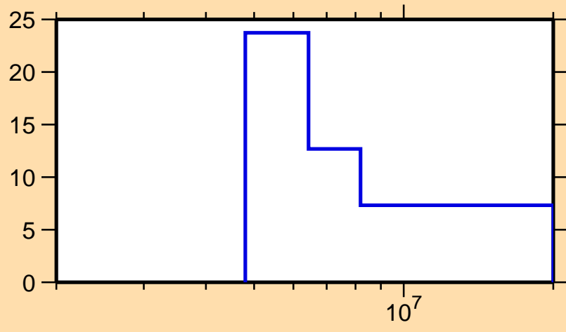
\Delta\sigma/\sigma vs. E for ^{147}\text{Nd}(n,2n)
