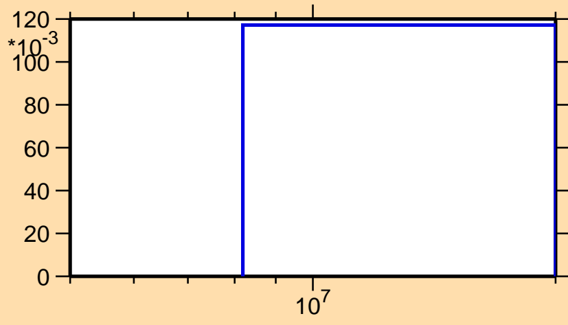
\sigma vs. E for ^{147}\text{Nd}(n,3n)
