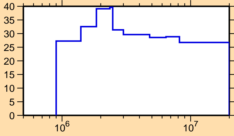
\Delta\sigma/\sigma vs. E for ^{147}\text{Nd}(n,n_1)
