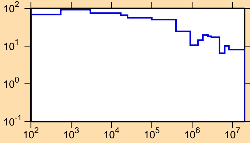
\Delta\sigma/\sigma vs. E for ^{147}\text{Nd}(n,\text{el.})
