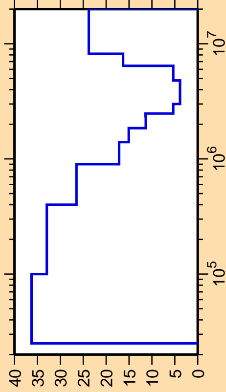
\Delta\sigma/\sigma vs. E for ^{147}\text{Nd}(n,\text{inel.})
