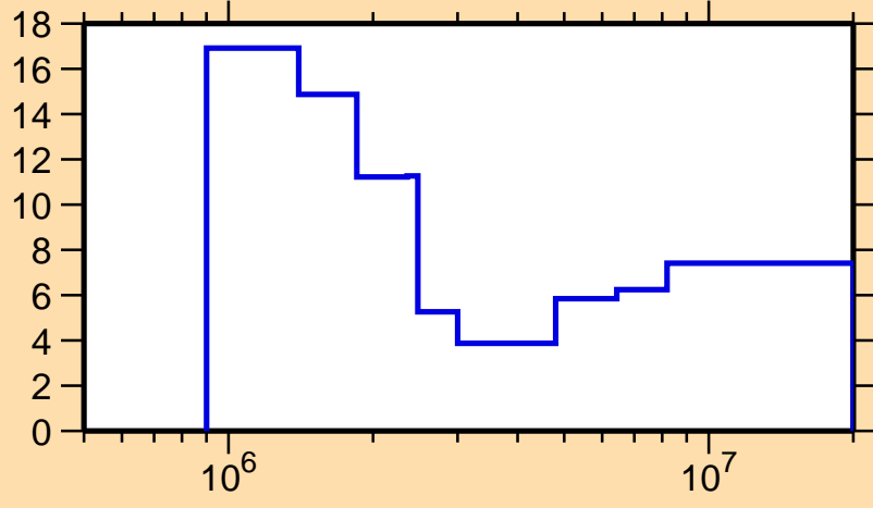
\Delta\sigma/\sigma vs. E for ^{147}\text{Nd}(n,n\text{onel.})
