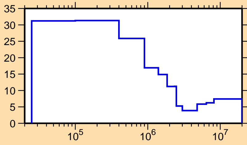
\Delta\sigma/\sigma vs. E for ^{147}\text{Nd}(n,\text{nonel.})
