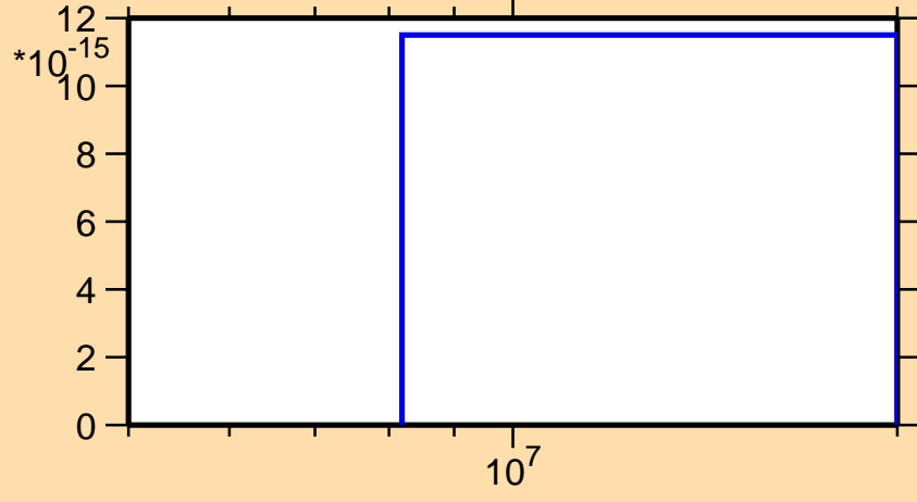
\sigma vs. E for ^{147}\text{Nd}(\text{mt117})
