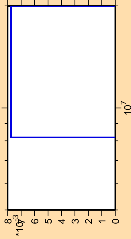
\Delta\sigma/\sigma vs. E for ^{147}\text{Nd}(\text{mt } 45)
