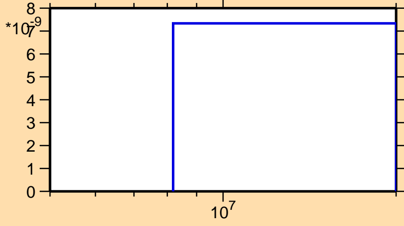
\sigma vs. E for ^{147}\text{Nd}(n,2np)
