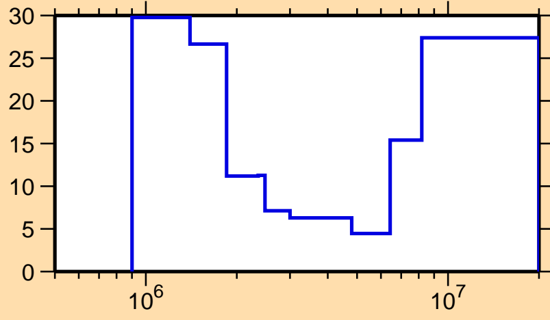
\Delta\sigma/\sigma vs. E for ^{147}\text{Nd}(n,n\text{cont.})
