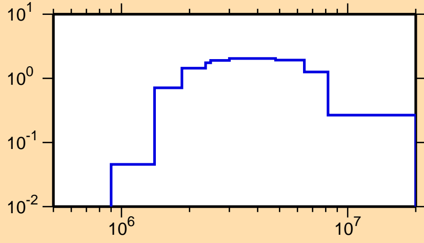
\sigma vs. E for ^{147}\text{Nd}(n,n\text{cont.})
