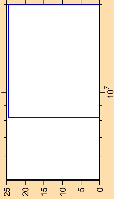
\Delta\sigma/\sigma vs. E for ^{147}\text{Nd}(n,3n)
