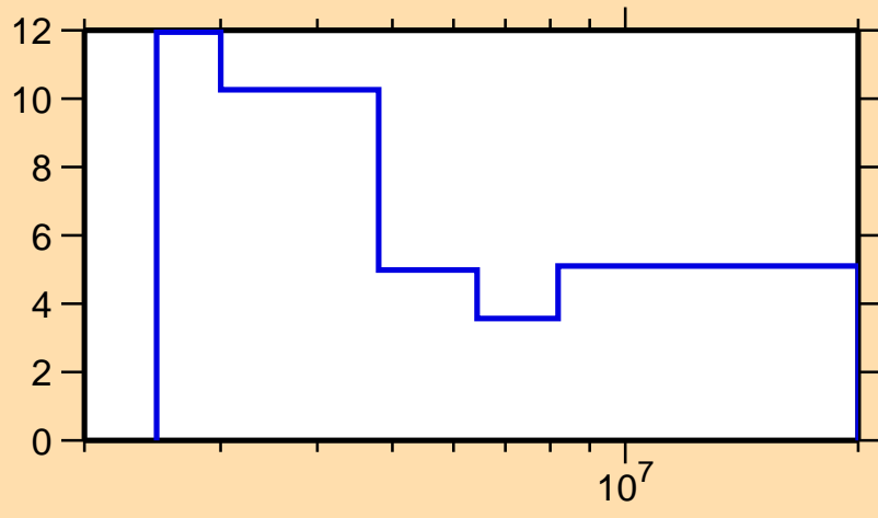
\Delta\sigma/\sigma vs. E for ^{147}\text{Nd}(n,\text{tot.})
