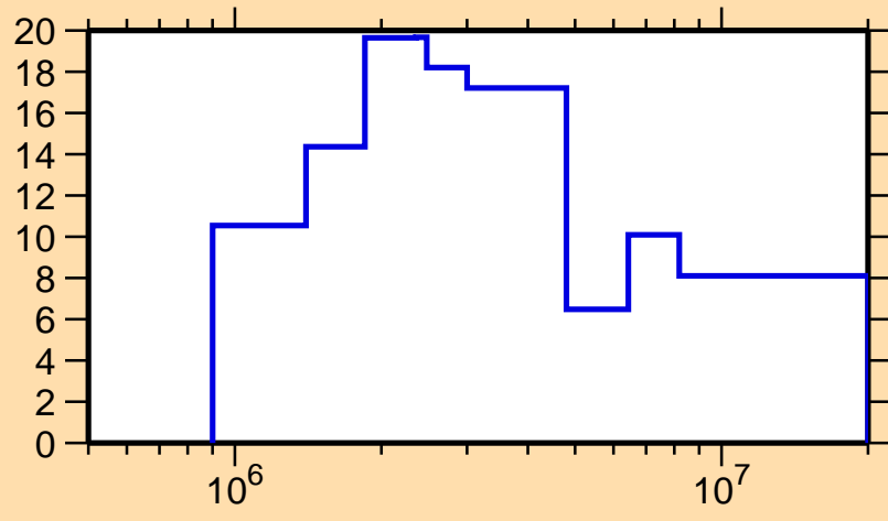
\Delta\sigma/\sigma vs. E for ^{147}\text{Nd}(n,\text{el.})
