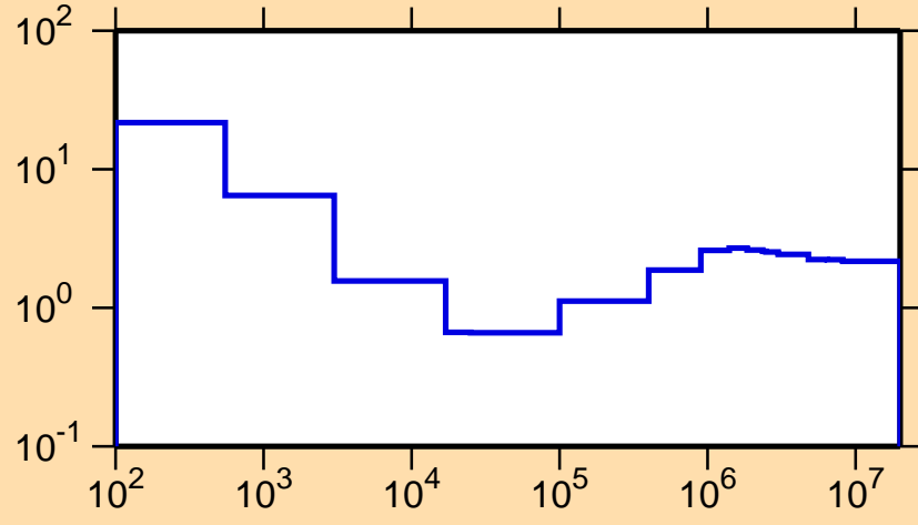
\sigma vs. E for ^{147}\text{Nd}(n,\text{nonel.})
