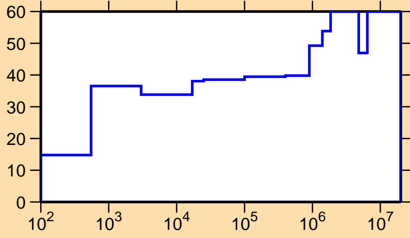
\Delta\sigma/\sigma vs. E for ^{147}\text{Nd}(n,\gamma)
