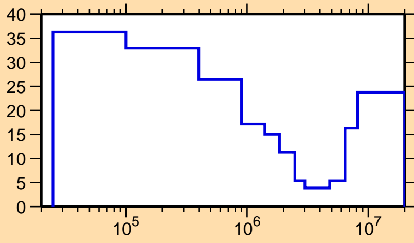
\Delta\sigma/\sigma vs. E for ^{147}\text{Nd}(n,\text{inel.})
