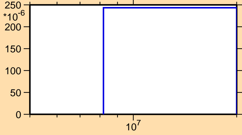
\sigma vs. E for ^{147}\text{Nd}(n,d)
