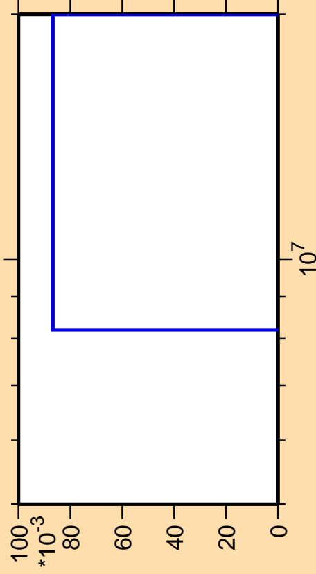
\Delta\sigma/\sigma vs. E for ^{147}\text{Nd}(\text{mt117})
