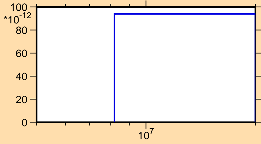
\sigma vs. E for ^{147}\text{Nd}(n,3n\alpha)
