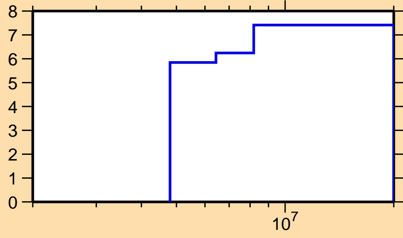
\Delta\sigma/\sigma vs. E for ^{147}\text{Nd}(n,\text{nonel.})
