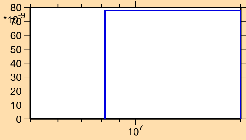
\sigma vs. E for ^{147}\text{Nd}(n,\text{nd})
