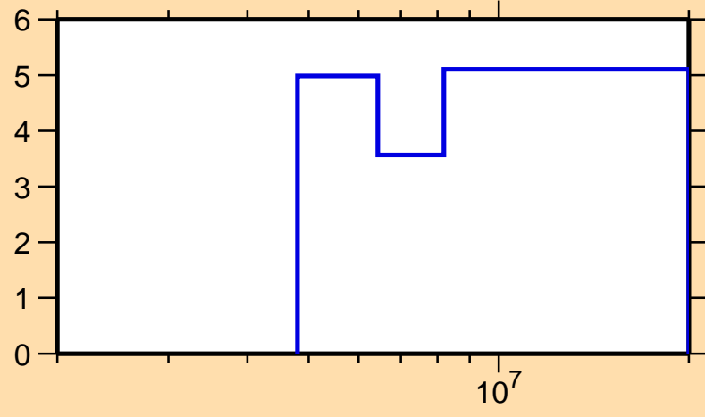
\Delta\sigma/\sigma vs. E for ^{147}\text{Nd}(n,\text{tot.})
