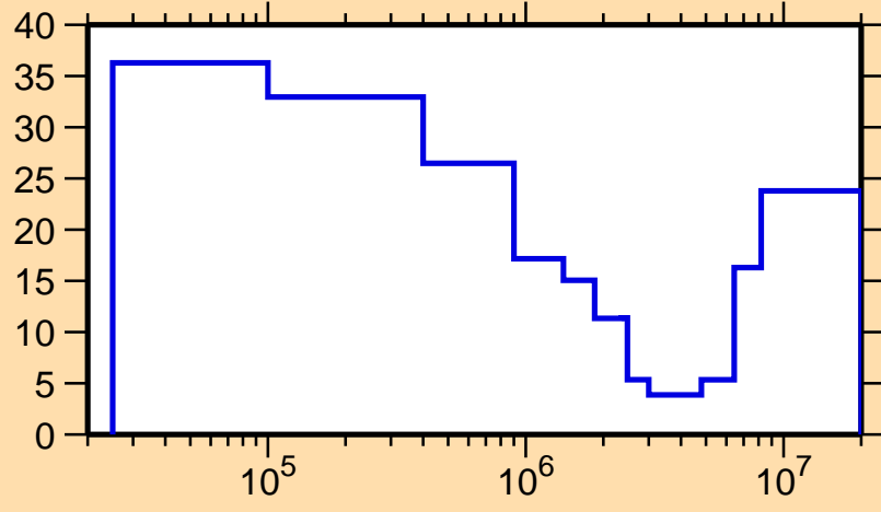
\Delta\sigma/\sigma vs. E for ^{147}\text{Nd}(n,\text{inel.})
