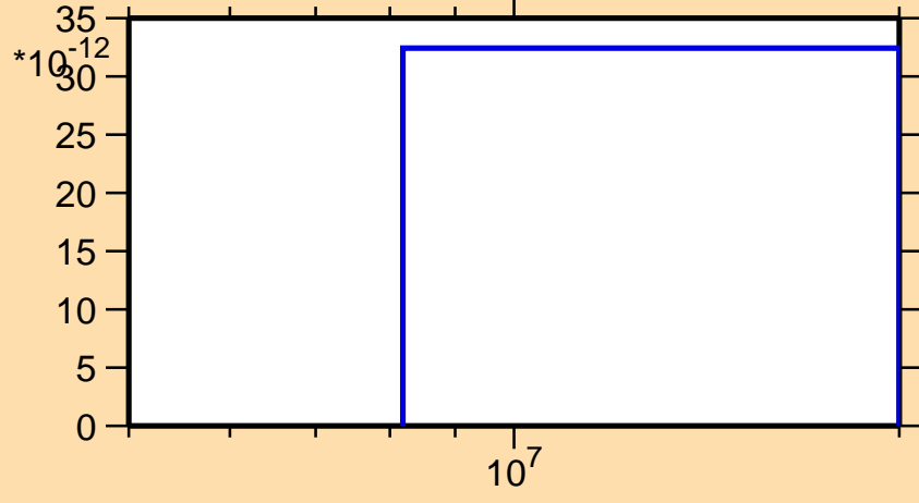
\sigma vs. E for ^{147}\text{Nd}(n,p\alpha)
