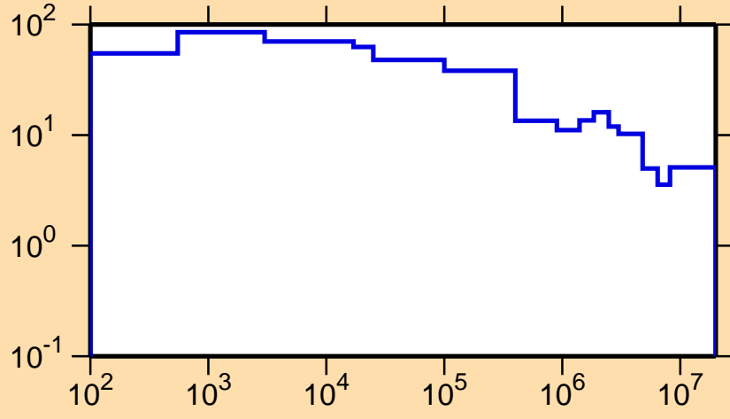
\Delta\sigma/\sigma vs. E for ^{147}\text{Nd}(n,\text{tot.})
