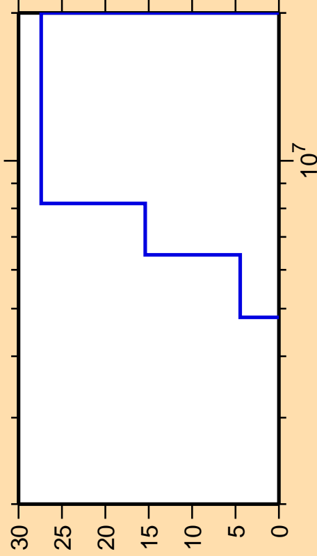
\Delta\sigma/\sigma vs. E for ^{147}\text{Nd}(n,n\text{cont.})
