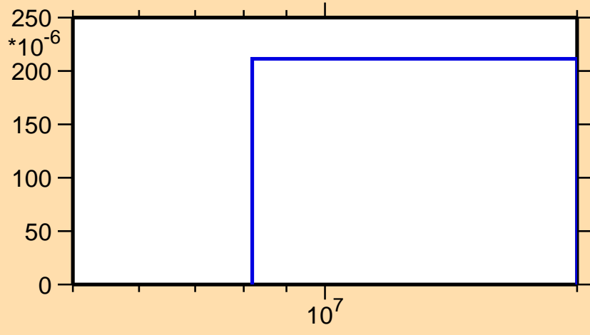
\sigma vs. E for ^{147}\text{Nd}(n,t)
