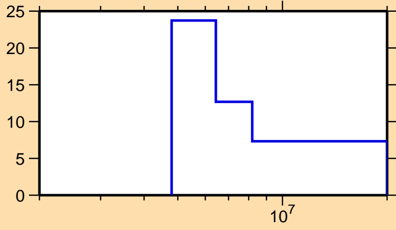
\Delta\sigma/\sigma vs. E for ^{147}\text{Nd}(n,2n)
