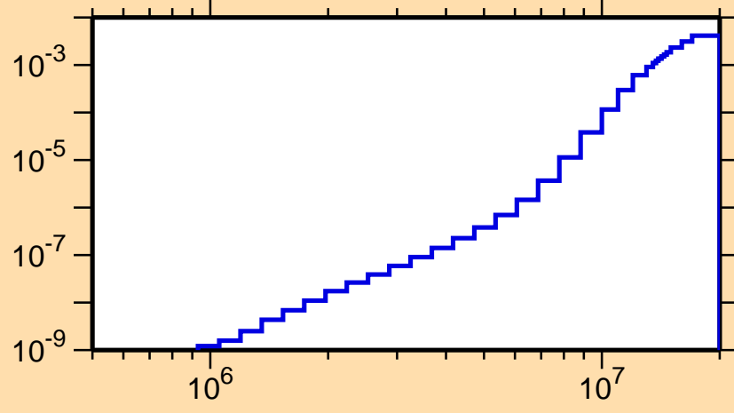
\sigma vs. E for ^{148}\text{Nd}(n,\alpha)
