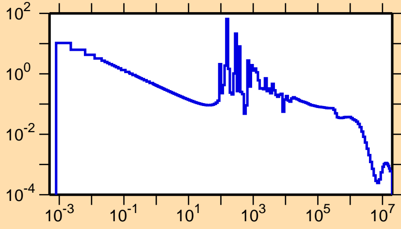
\sigma vs. E for ^{148}\text{Nd}(n,\gamma)
