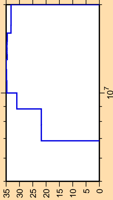
\Delta\sigma/\sigma vs. E for ^{148}\text{Nd}(n,n\text{cont.})
