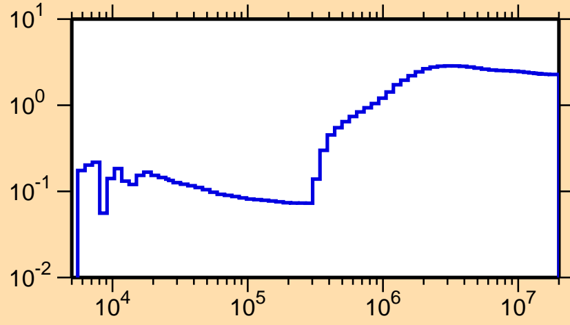
\sigma vs. E for ^{148}\text{Nd}(n,\text{nonel.})
