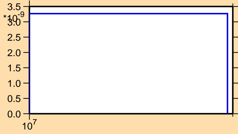
\sigma vs. E for ^{148}\text{Nd}(n,nt)
