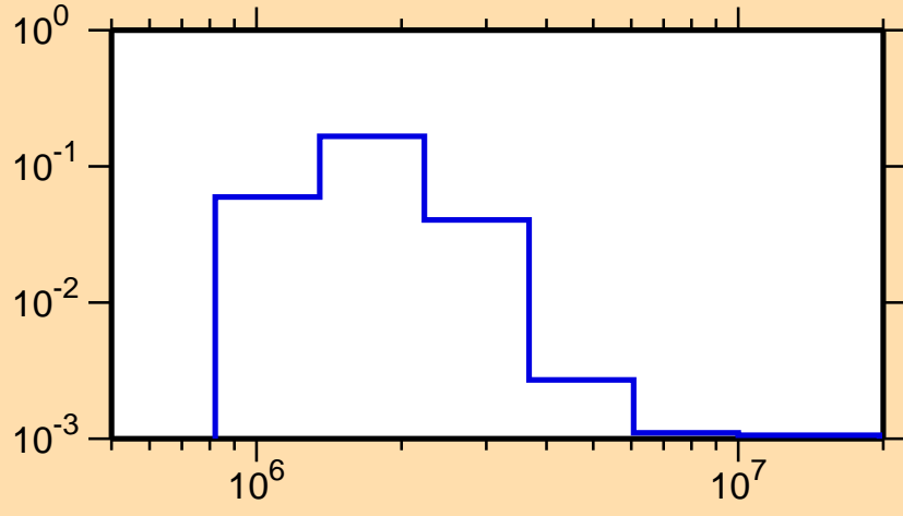
\sigma vs. E for ^{148}\text{Nd}(n,n_4)
