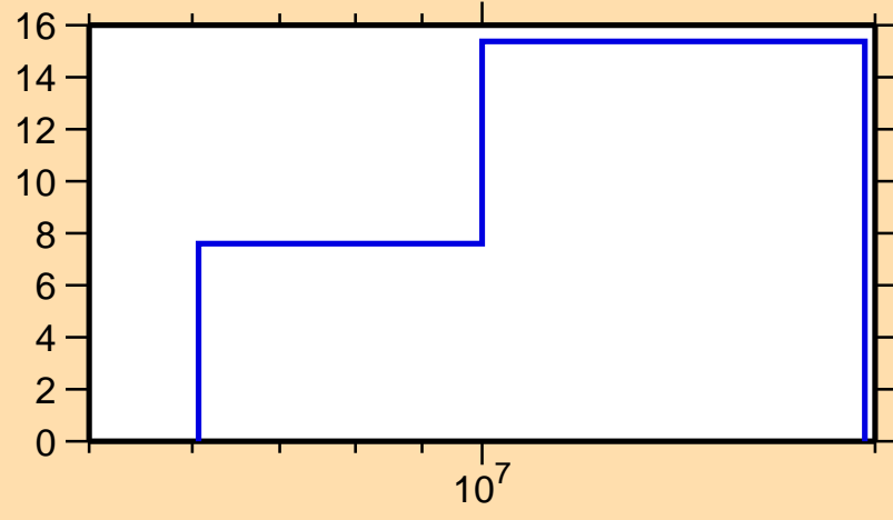
\Delta\sigma/\sigma vs. E for ^{148}\text{Nd}(n,2n)
