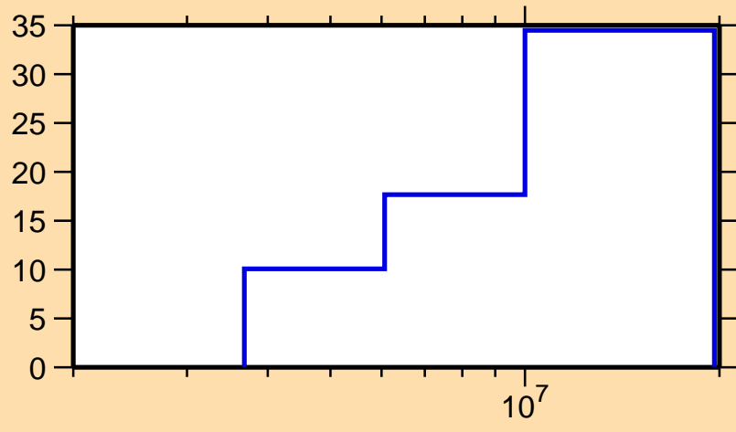
\Delta\sigma/\sigma vs. E for ^{148}\text{Nd}(n,n\text{cont.})
