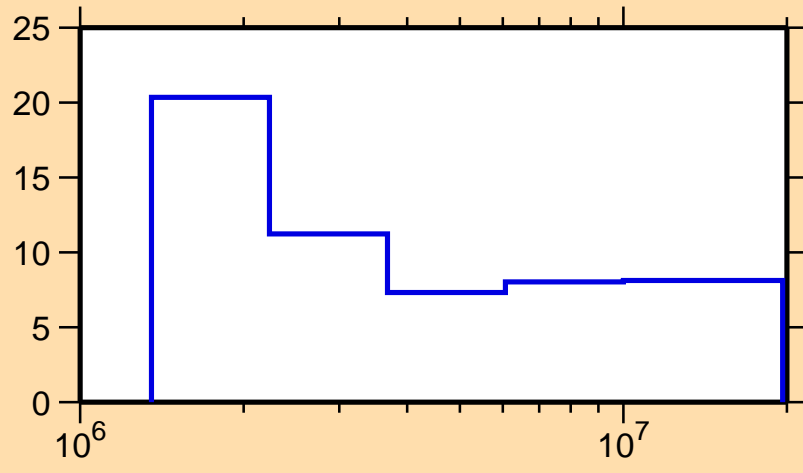
\Delta\sigma/\sigma vs. E for ^{148}\text{Nd}(n,n\text{onel.})
