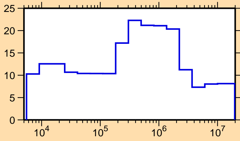
\Delta\sigma/\sigma vs. E for ^{148}\text{Nd}(n,\text{nonel.})
