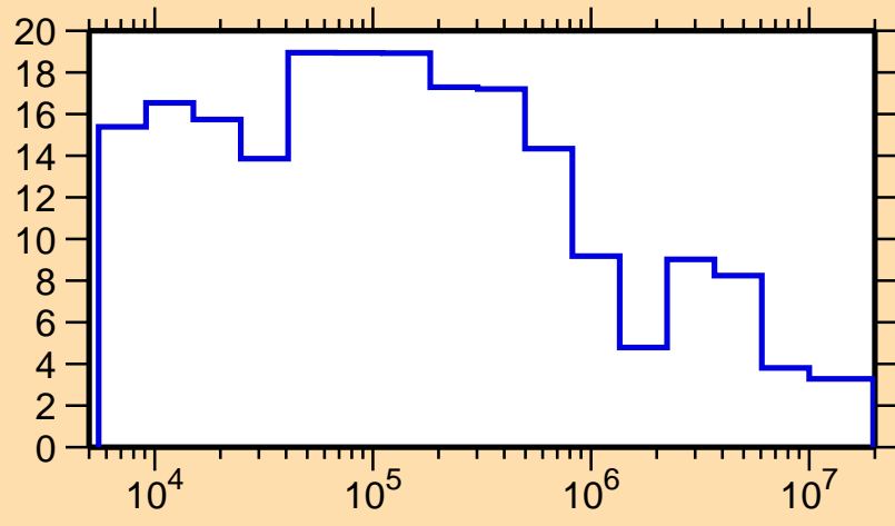
\Delta\sigma/\sigma vs. E for ^{148}\text{Nd}(n,\text{el.})
