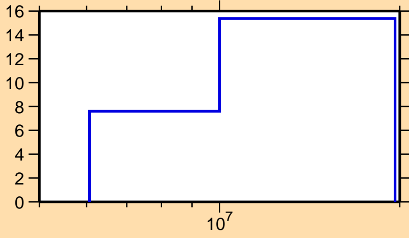
\Delta\sigma/\sigma vs. E for ^{148}\text{Nd}(n,2n)
