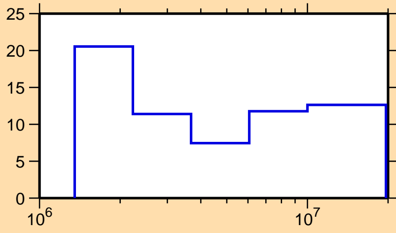
\Delta\sigma/\sigma vs. E for ^{148}\text{Nd}(n,\text{inel.})
