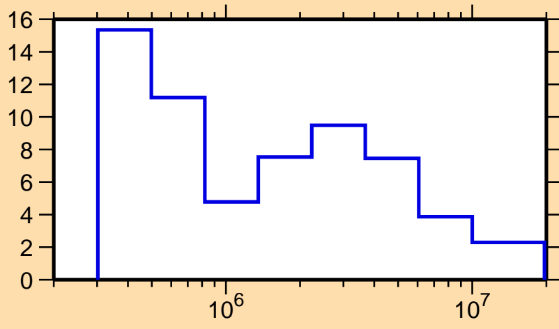
\Delta\sigma/\sigma vs. E for ^{148}\text{Nd}(n,\text{tot.})
