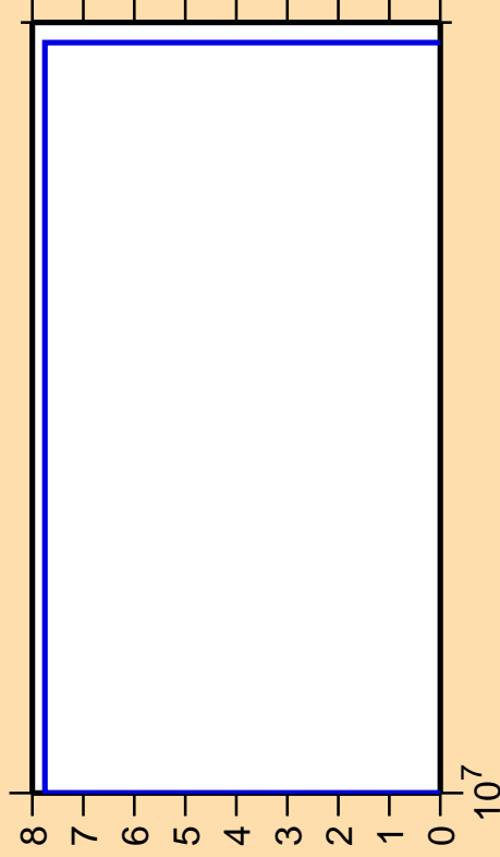
\Delta\sigma/\sigma vs. E for ^{148}\text{Nd}(n,3n)
