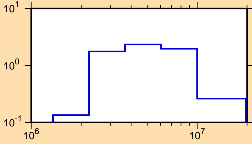
\sigma vs. E for ^{148}\text{Nd}(n,n\text{cont.})
