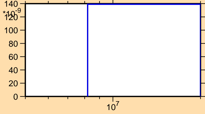
\sigma vs. E for ^{148}\text{Nd}(n,2n\alpha)
