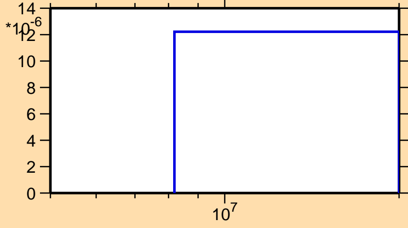
\sigma vs. E for ^{148}\text{Nd}(n,t)
