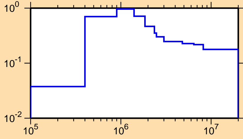
\sigma vs. E for ^{148}\text{Nd}(n,n_1)
