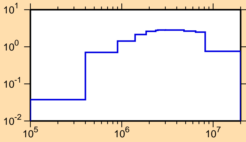
\sigma vs. E for ^{148}\text{Nd}(n,\text{inel.})
