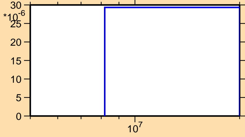
\sigma vs. E for ^{148}\text{Nd}(n,np)
