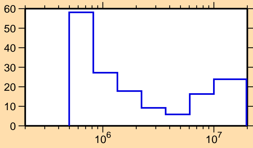
\Delta\sigma/\sigma vs. E for ^{149}\text{Nd}(n,n\text{cont.})
