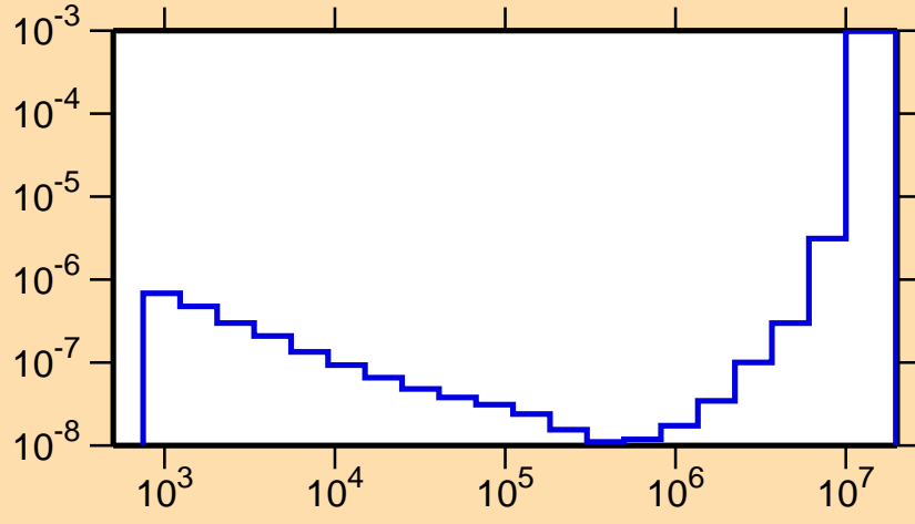
\sigma vs. E for ^{149}\text{Nd}(n,\alpha)
