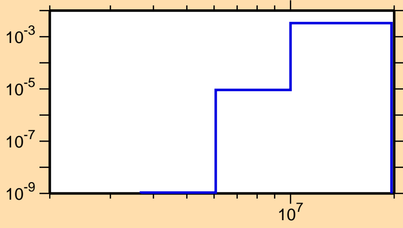
\sigma vs. E for ^{149}\text{Nd}(n,p)
