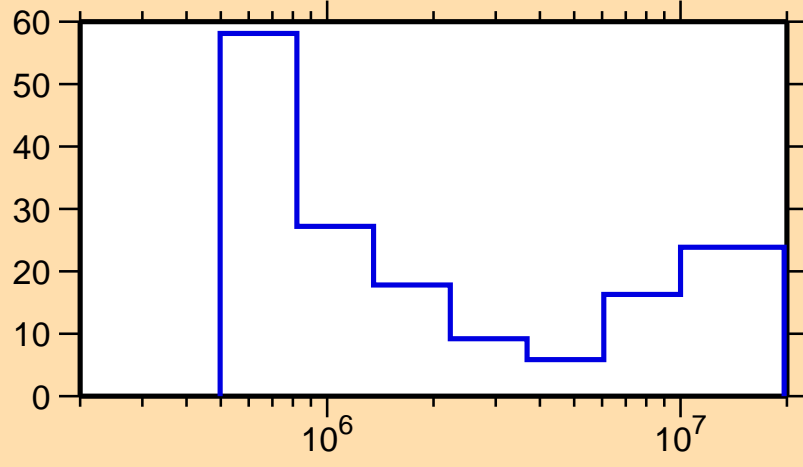
\Delta\sigma/\sigma vs. E for ^{149}\text{Nd}(n,n\text{cont.})
