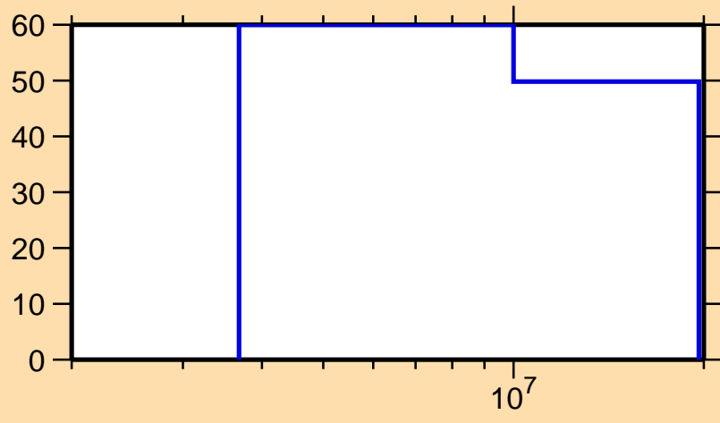
\Delta\sigma/\sigma vs. E for ^{149}\text{Nd}(n,p)
