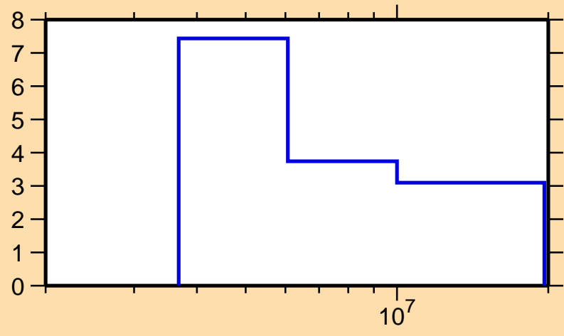
\Delta\sigma/\sigma vs. E for ^{149}\text{Nd}(n,\text{tot.})
