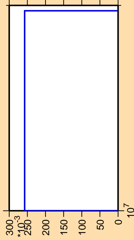
\Delta\sigma/\sigma vs. E for ^{149}\text{Nd}(n,p\alpha)
