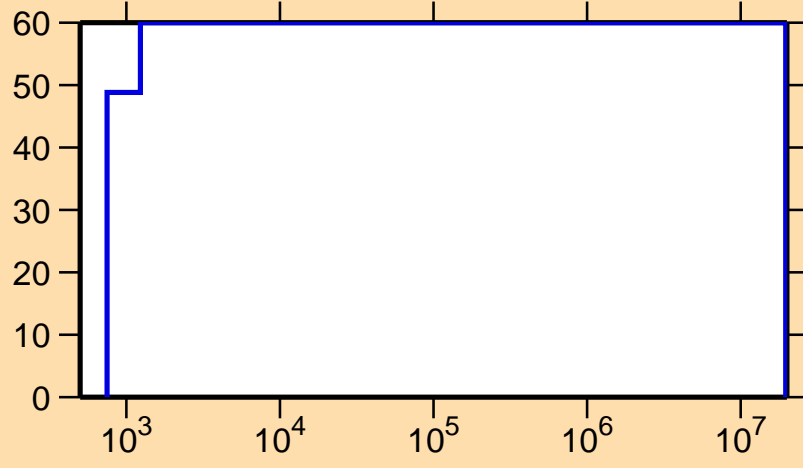
\Delta\sigma/\sigma vs. E for ^{149}\text{Nd}(n,\gamma)
