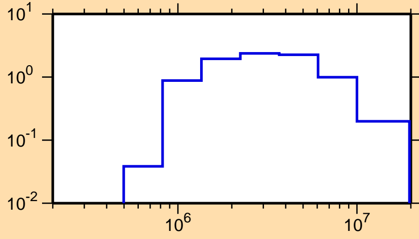
\sigma vs. E for ^{149}\text{Nd}(n,n\text{cont.})
