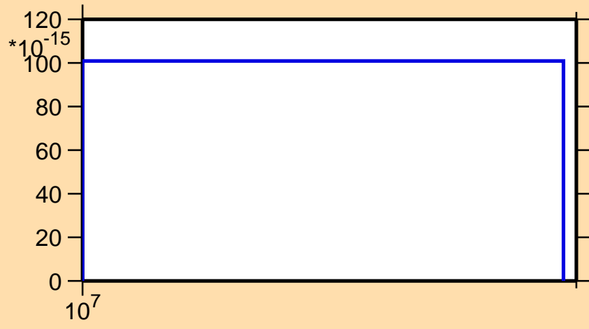
\sigma vs. E for ^{149}\text{Nd}(n,p\alpha)
