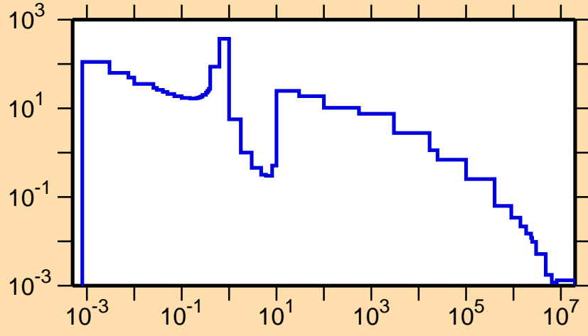
\sigma vs. E for ^{149}\text{Nd}(n,\gamma)
