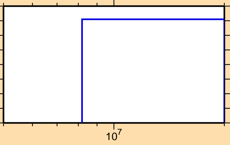
\sigma vs. E for ^{149}\text{Nd}(n,t)
