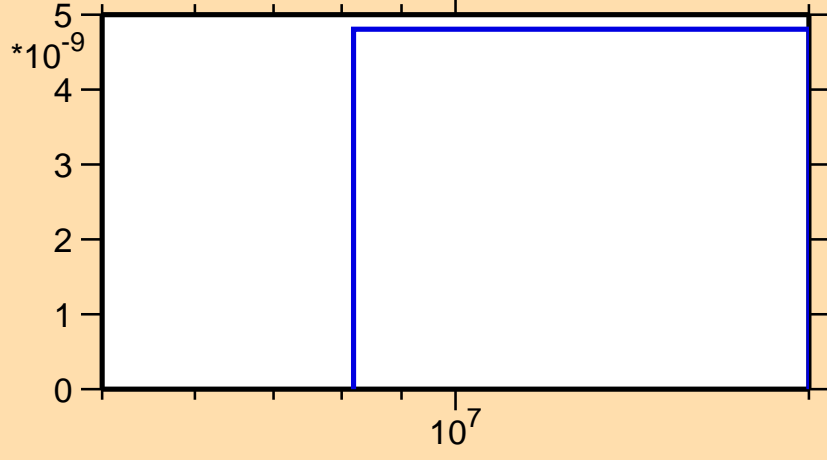
\sigma vs. E for ^{149}\text{Nd}(n,nt)
