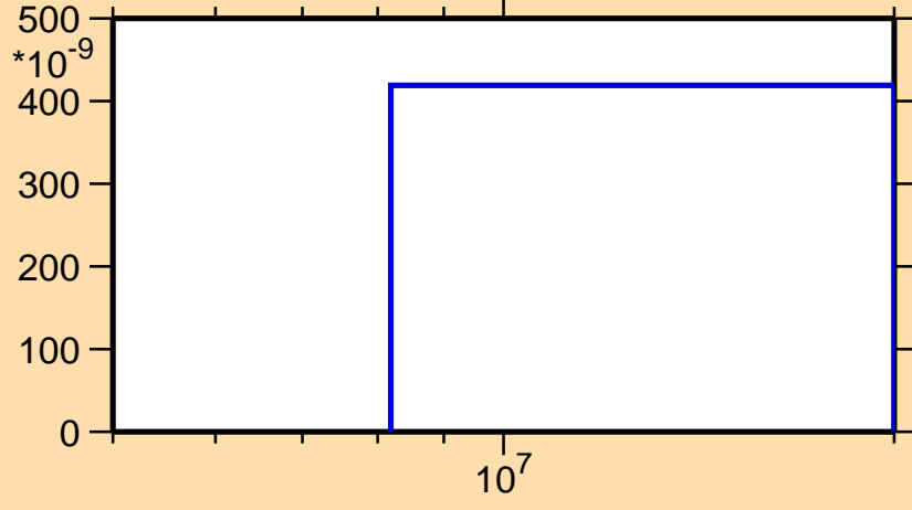
\sigma vs. E for ^{149}\text{Nd}(n,2n\alpha)
