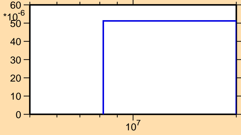
\sigma vs. E for ^{149}\text{Nd}(n,np)
