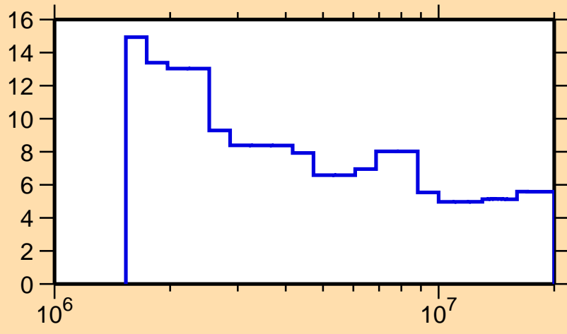
\Delta\sigma/\sigma vs. E for ^{150}\text{Nd}(n,n\text{onel.})
