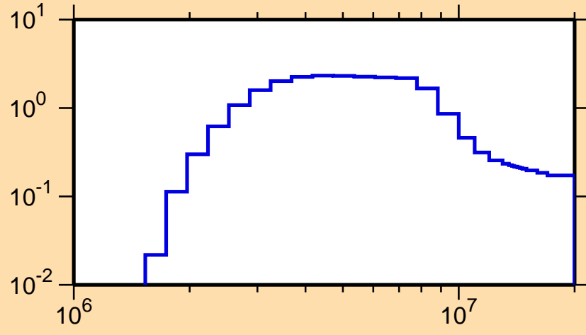
\sigma vs. E for ^{150}\text{Nd}(n,n\text{cont.})
