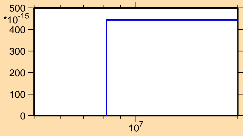
\sigma vs. E for ^{150}\text{Nd}(n,3n\alpha)
