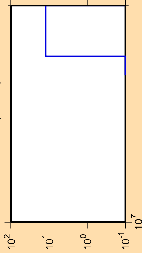
\Delta\sigma/\sigma vs. E for ^{151}\text{Nd}(n,3n\alpha)
