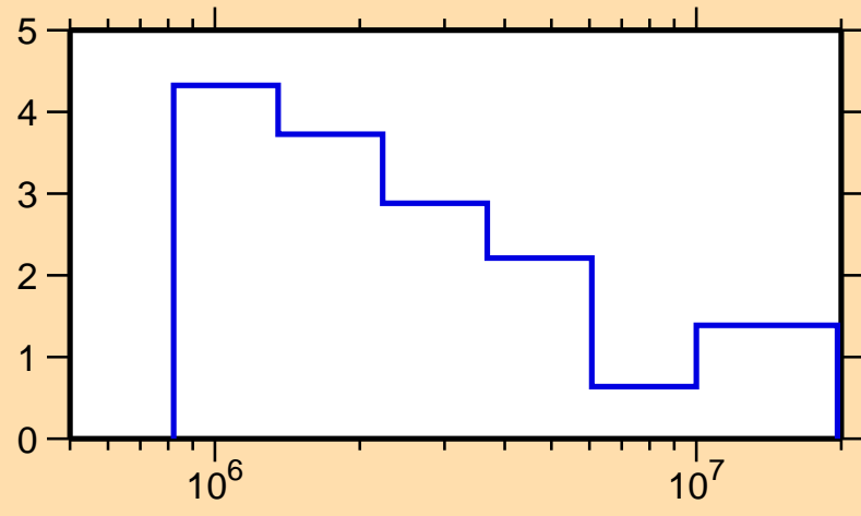
\Delta\sigma/\sigma vs. E for ^{151}\text{Nd}(n,\text{tot.})
