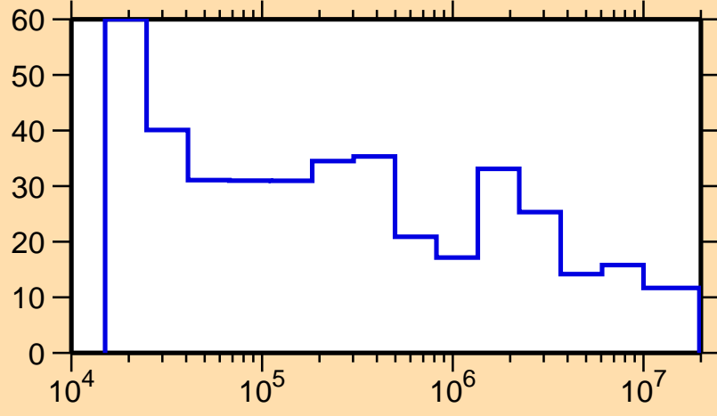
\Delta\sigma/\sigma vs. E for ^{151}\text{Nd}(n,n_1)
