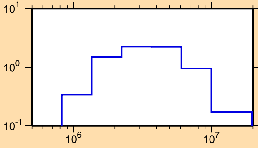
\sigma vs. E for ^{151}\text{Nd}(n,n\text{cont.})
