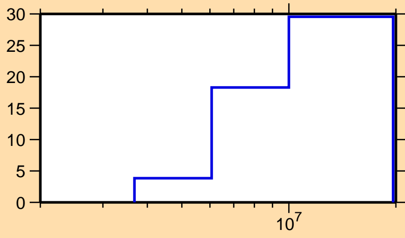
\Delta\sigma/\sigma vs. E for ^{151}\text{Nd}(n,n\text{cont.})
