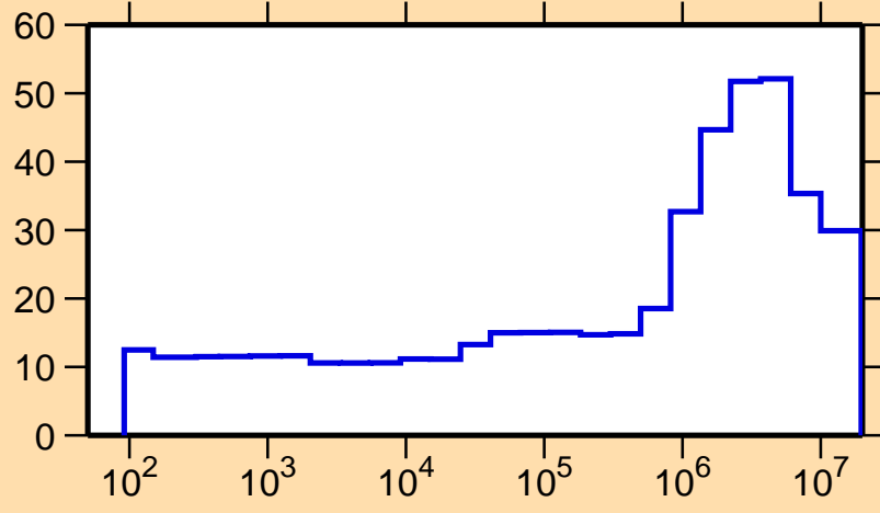
\Delta\sigma/\sigma vs. E for ^{151}\text{Nd}(n,\gamma)
