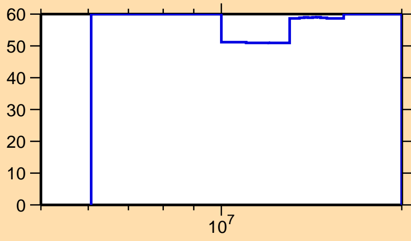
\Delta\sigma/\sigma vs. E for ^{152}\text{Nd}(n,\gamma)
