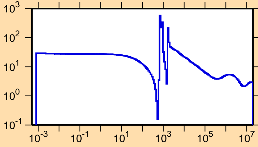
\sigma vs. E for ^{152}\text{Nd}(n,\text{el.})
