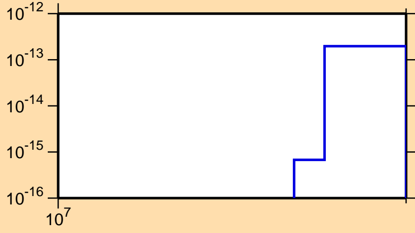
\sigma vs. E for ^{152}\text{Nd}(n,3n\alpha)
