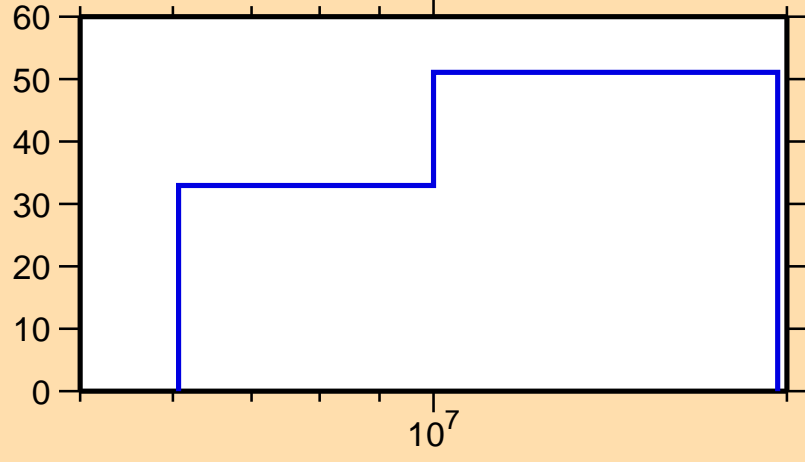
\Delta\sigma/\sigma vs. E for ^{153}\text{Nd}(n,ncont.)
