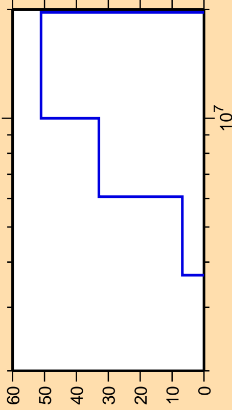
\Delta\sigma/\sigma vs. E for ^{153}\text{Nd}(n,n\text{cont.})
