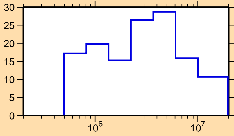
\Delta\sigma/\sigma vs. E for ^{153}\text{Nd}(n,\text{tot.})
