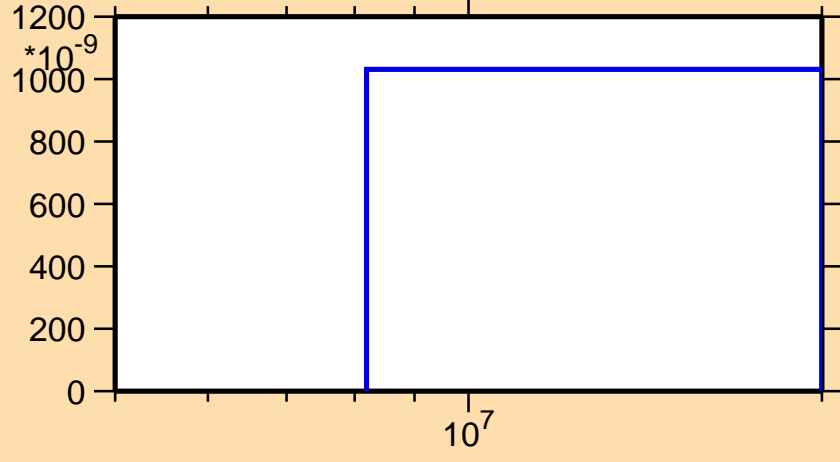
\sigma vs. E for ^{153}\text{Nd}(n,n\alpha)
