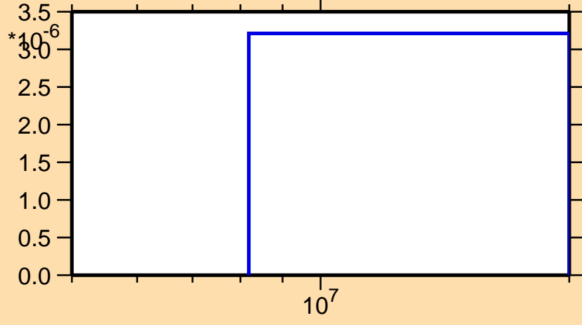
\sigma vs. E for ^{153}\text{Nd}(n,t)
