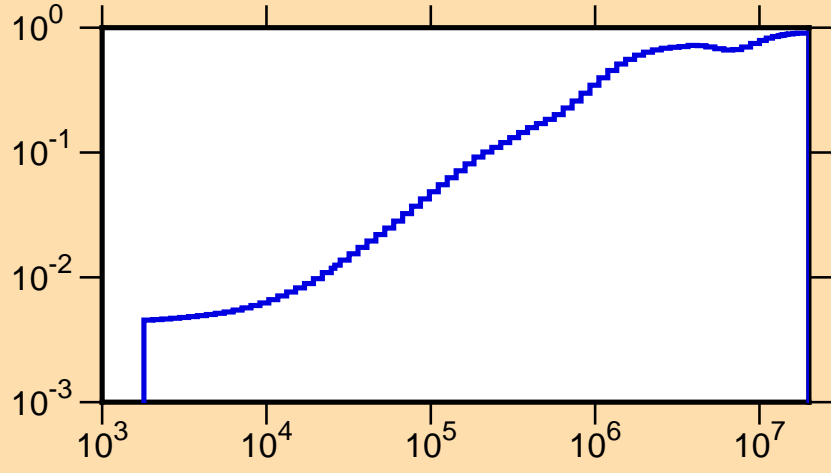
\mu vs. E for ^{154}\text{Nd}(\text{mt251})
