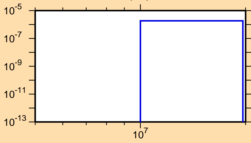
\sigma vs. E for ^{154}\text{Nd}(n,t)
