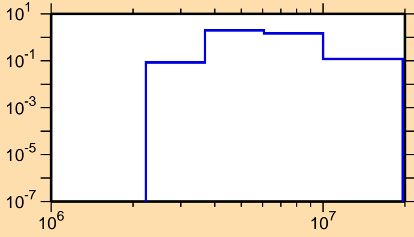
\sigma vs. E for ^{154}\text{Nd}(n,n\text{cont.})
