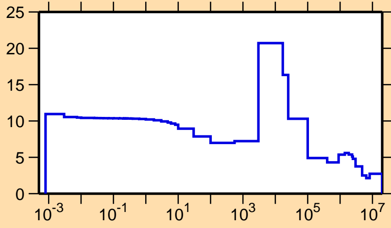
\sigma vs. E for ^{154}\text{Nd}(n,\text{el.})
