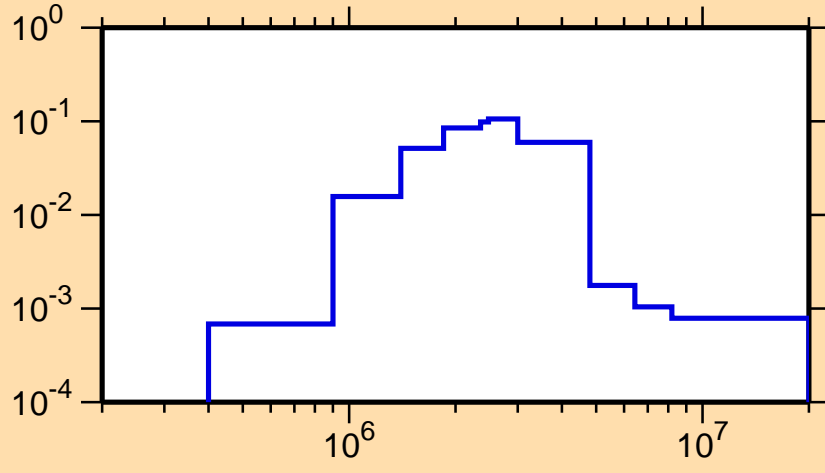
\sigma vs. E for ^{154}\text{Nd}(n,n_3)
