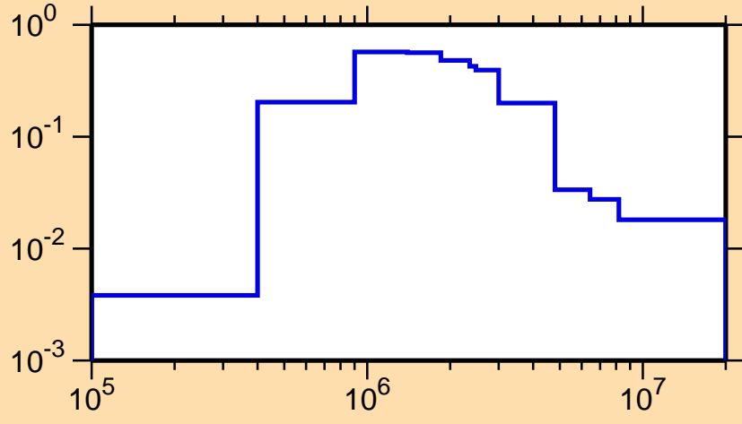
\sigma vs. E for ^{154}\text{Nd}(n,n_2)
