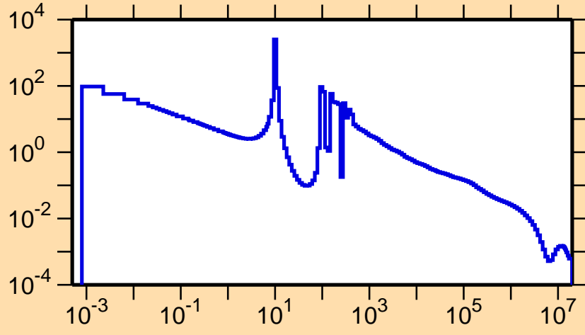
\sigma vs. E for ^{155}\text{Nd}(n,\gamma)
