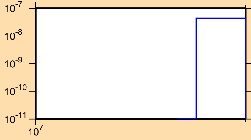
\sigma vs. E for ^{155}\text{Nd}(n,nt)
