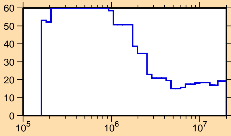
\Delta\sigma/\sigma vs. E for ^{155}\text{Nd}(n,\text{nonel.})
