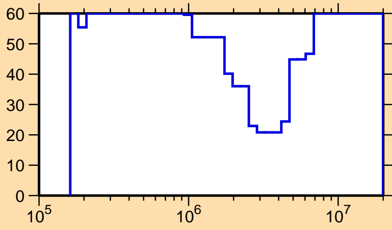
\Delta\sigma/\sigma vs. E for ^{155}\text{Nd}(n,\text{inel.})
