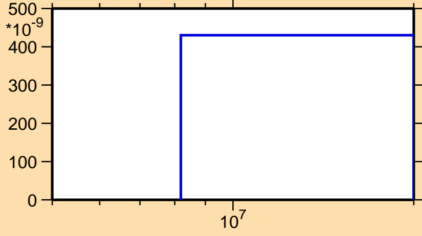
\sigma vs. E for ^{155}\text{Nd}(n,n\alpha)
