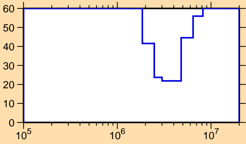
\Delta\sigma/\sigma vs. E for ^{155}\text{Nd}(n,n\text{cont.})
