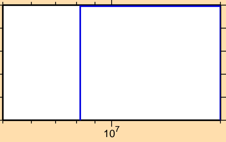
\sigma vs. E for ^{155}\text{Nd}(n,t)
