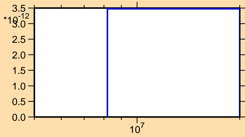
\sigma vs. E for ^{155}\text{Nd}(n,2np)
