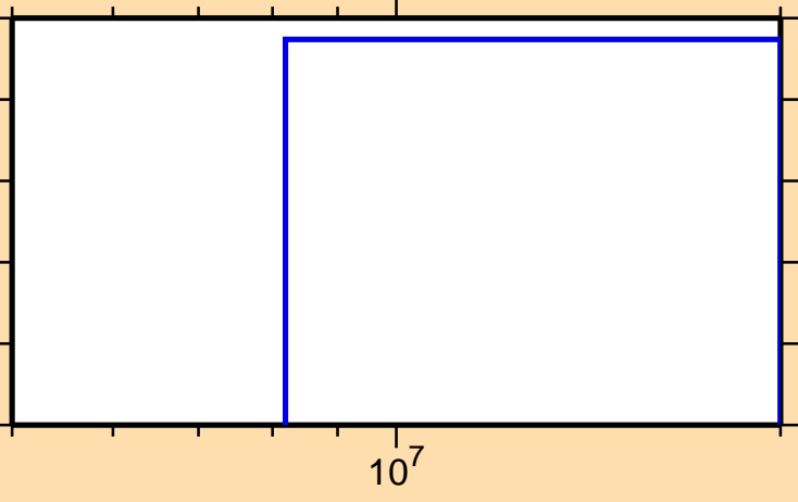
\sigma vs. E for ^{155}\text{Nd}(n,np)
