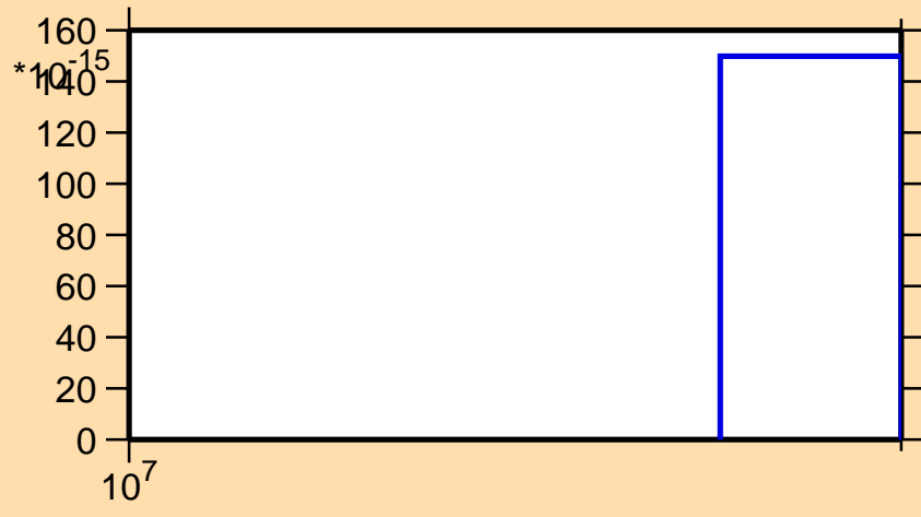
\sigma vs. E for ^{156}\text{Nd}(n,2np)
