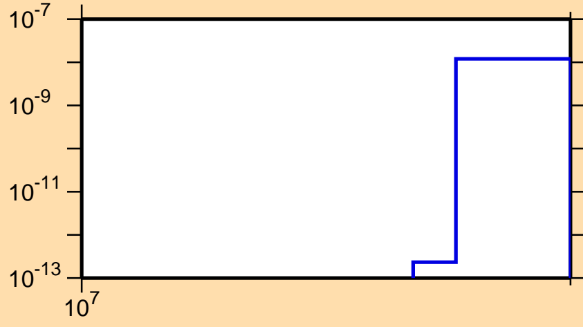
\sigma vs. E for ^{156}\text{Nd}(n,nt)
