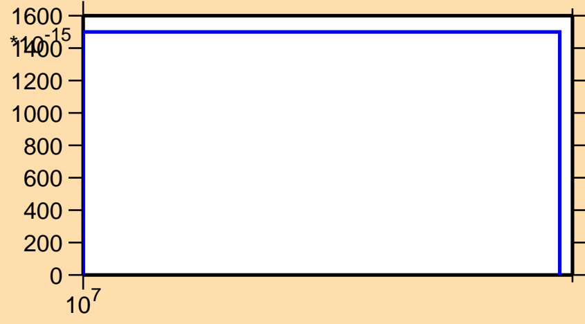
\sigma vs. E for ^{156}\text{Nd}(n,nd)
