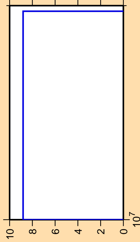
\Delta\sigma/\sigma vs. E for ^{156}\text{Nd}(n,nd)
