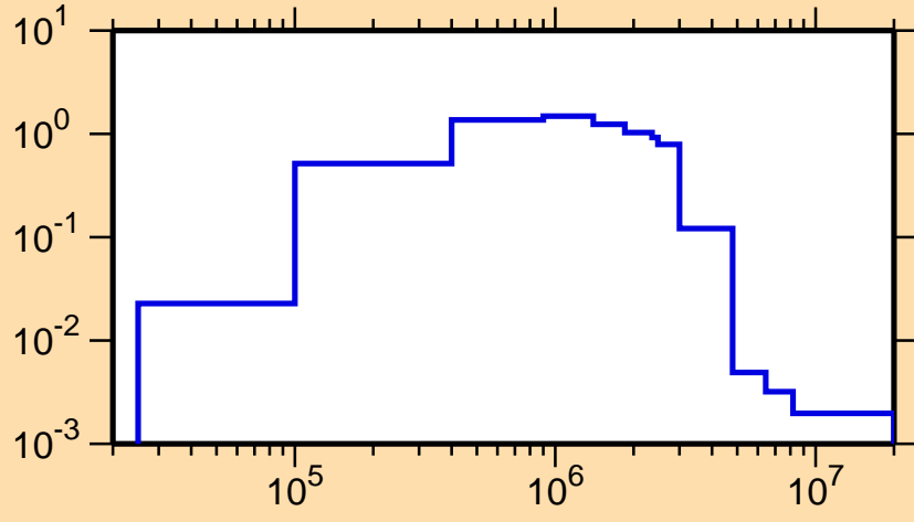
\sigma vs. E for ^{156}\text{Nd}(n,n_1)
