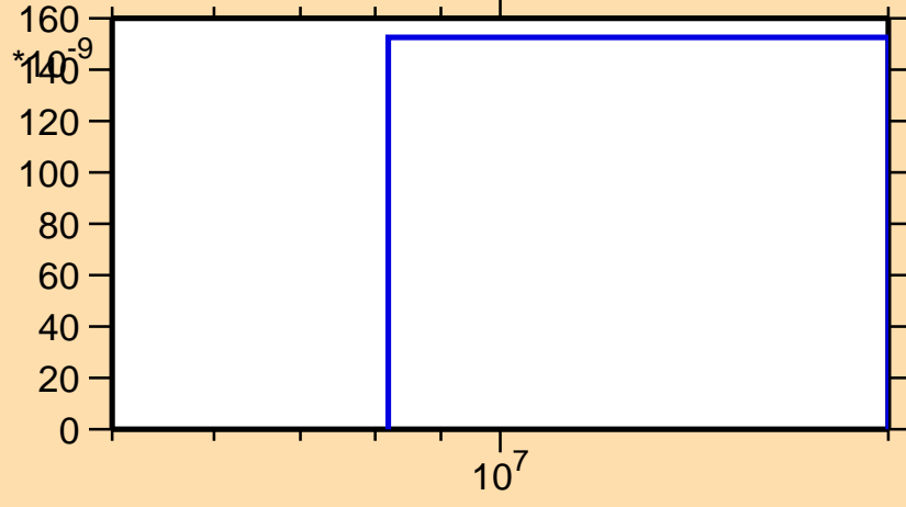
\sigma vs. E for ^{156}\text{Nd}(n,n\alpha)
