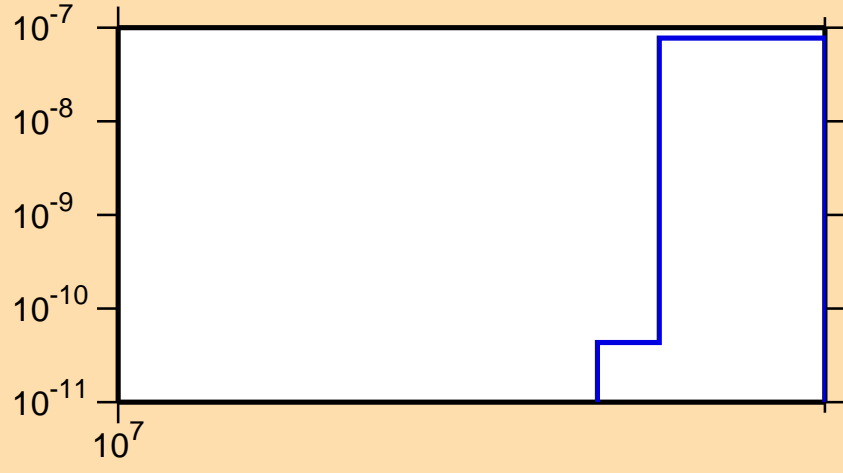
\sigma vs. E for ^{157}\text{Nd}(n,nt)
