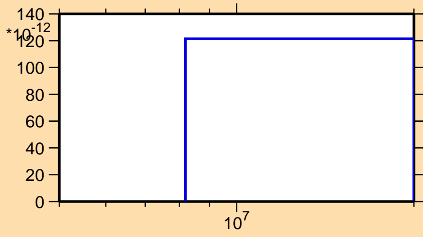
\sigma vs. E for ^{157}\text{Nd}(n,\text{nd})
