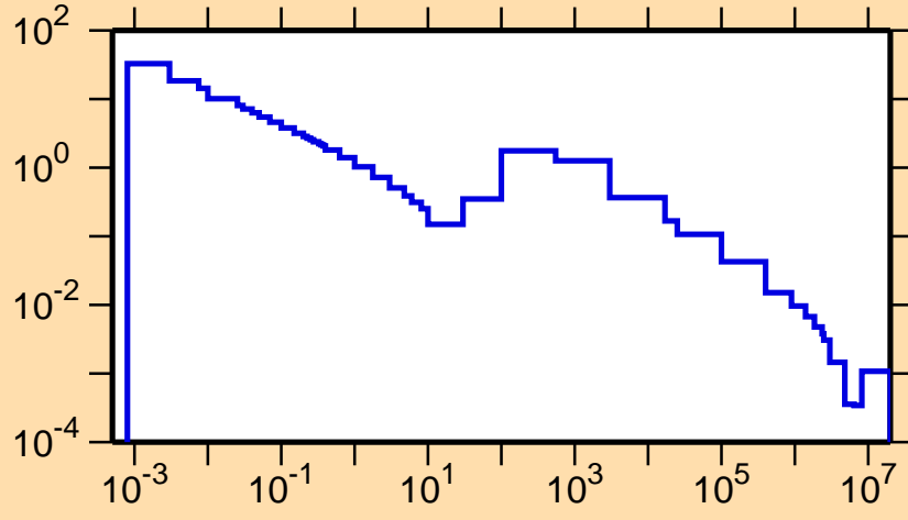
\sigma vs. E for ^{157}\text{Nd}(n,\gamma)
