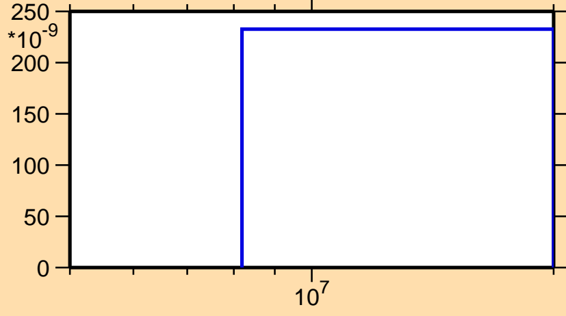
\sigma vs. E for ^{157}\text{Nd}(n,n\alpha)
