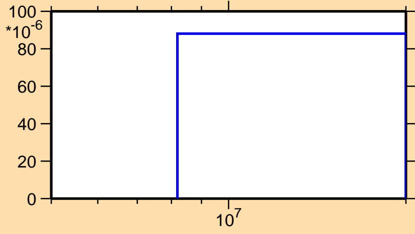
\sigma vs. E for ^{157}\text{Nd}(n,p)
