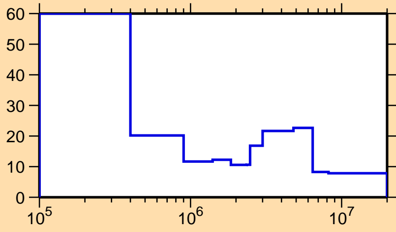
\Delta\sigma/\sigma vs. E for ^{157}\text{Nd}(n,\text{el.})
