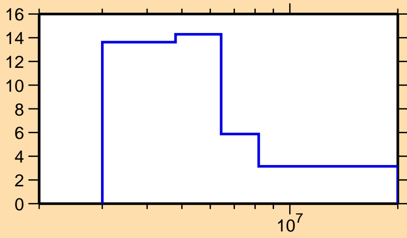
\Delta\sigma/\sigma vs. E for ^{157}\text{Nd}(n,\text{tot.})
