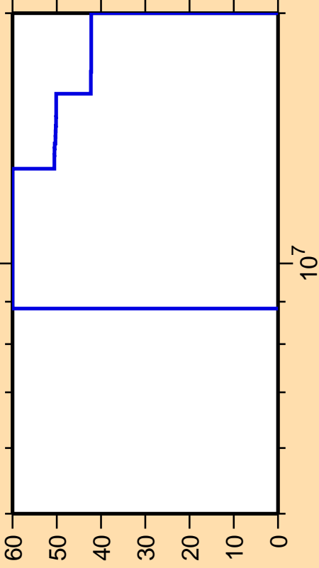
\Delta\sigma/\sigma vs. E for ^{18}\text{Ne}(\text{mt117})
