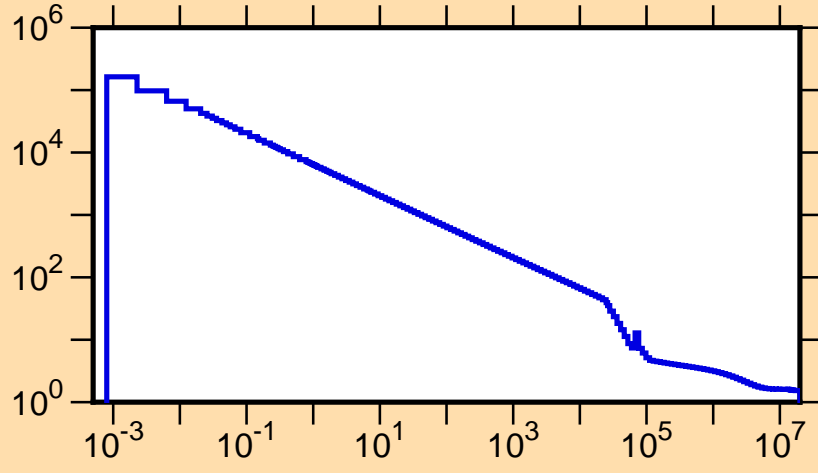
\sigma vs. E for ^{18}\text{Ne}(n,\text{tot.})
