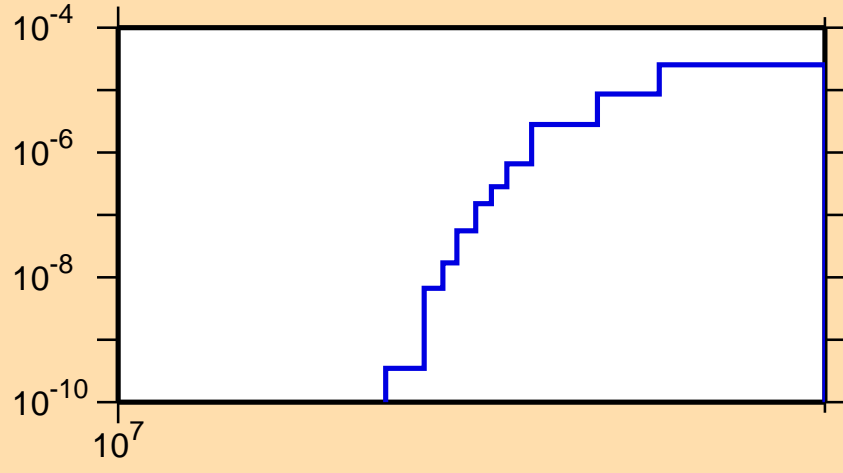
\sigma vs. E for ^{18}\text{Ne}(n,\text{pt})
